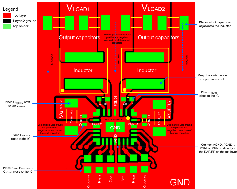
Figure 8-71. Layout Example
