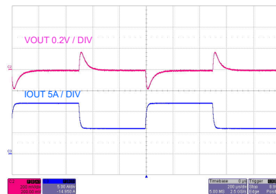
V_{OUT} = 3.3\text{ V} F_{SW} = 400\text{ kHz} FPWM mode I_{OUT} = 6\text{ A to }12\text{ A to }6\text{ A} V_{IN} = 13.5\text{ V} Single Output
