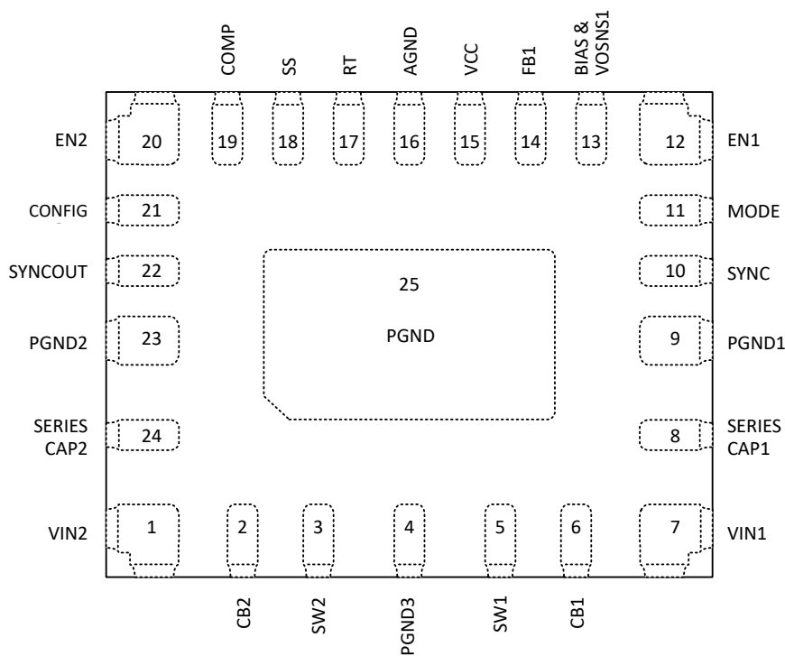
Figure 5-3. Single Output Secondary (Top View)
