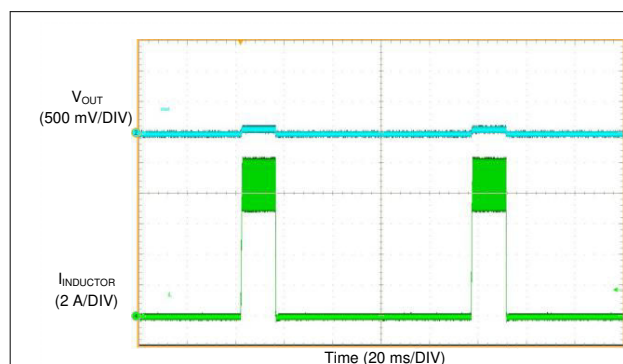
Figure 8-20. Inductor Current Bursts During Hiccup
