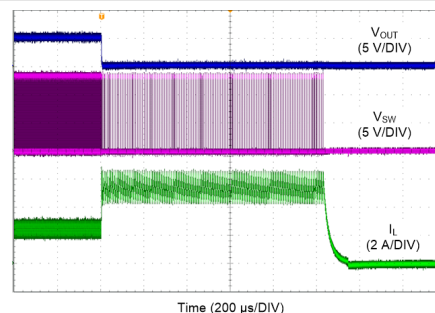
Figure 9-18. LMQ62440-Q1 Switching Waveform and V_{OUT} Ripple
