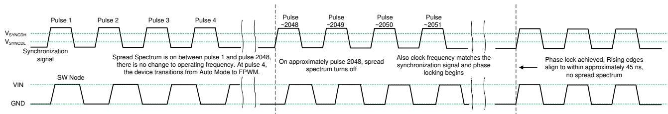
Figure 8-12. Synchronization Process
