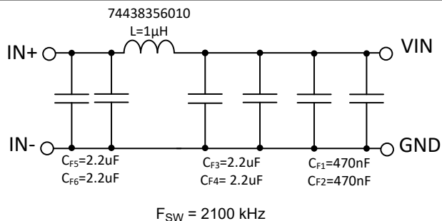
Figure 9-41. Recommended Input EMI Filter
