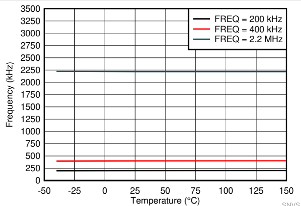
Figure 7-4. Switching Frequency
