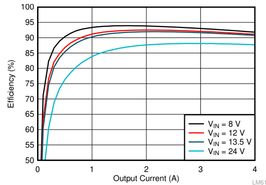
Figure 9-6. LMQ62440-Q1 Efficiency
