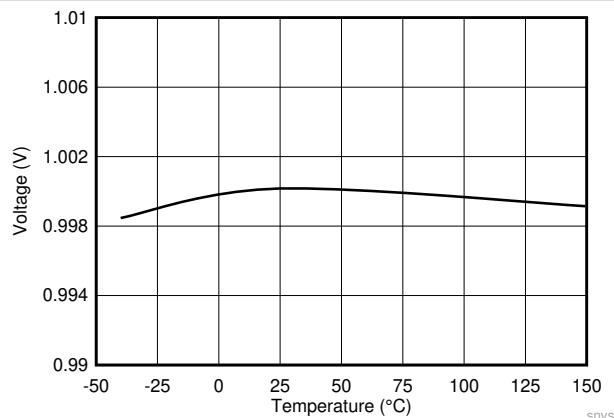
Figure 7-3. Feedback Voltage
