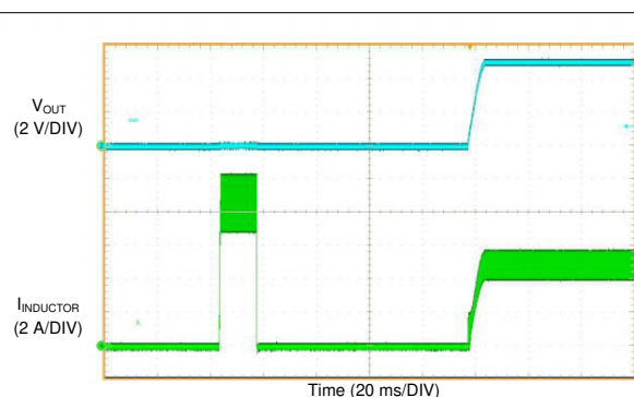
Figure 8-21. Short-Circuit Recovery
