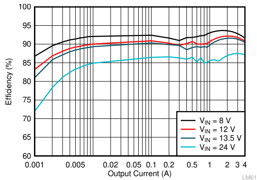
Figure 9-5. LMQ62440-Q1 Efficiency
