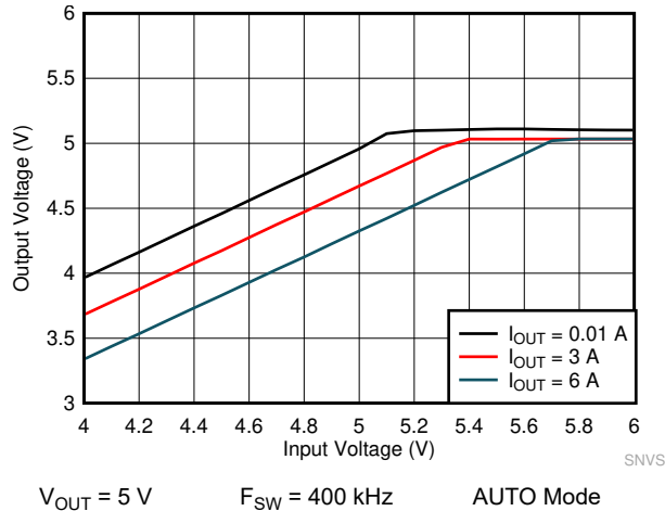
Figure 10-23. LMQ61460-Q1 Dropout Curve
