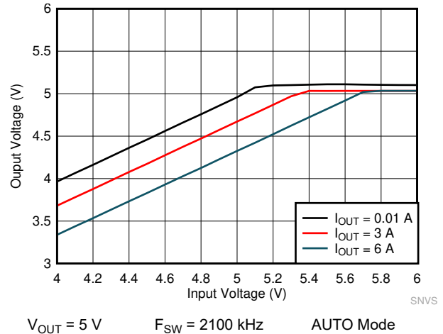
Figure 10-24. LMQ61460-Q1 Dropout Curve
