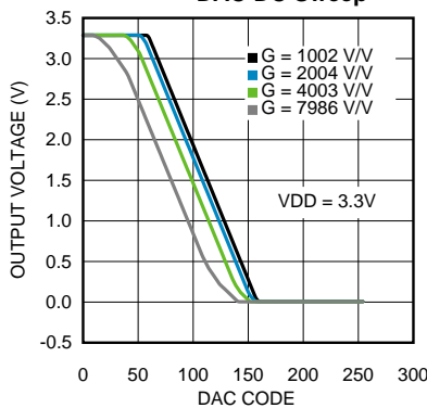
DAC DC Sweep
