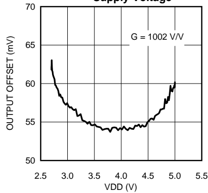
Output Offset vs Supply Voltage
