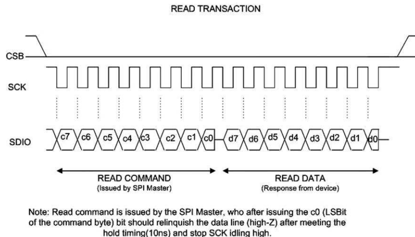
Figure 10. Read Transaction
