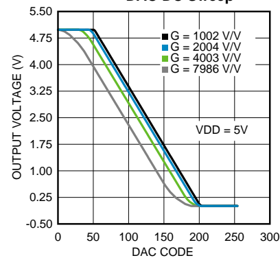
DAC DC Sweep
