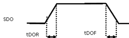
Figure 7. SDO Rise and Fall Times
