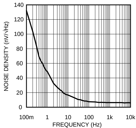
Figure 30. Input-Referred Noise Density vs. Frequency
