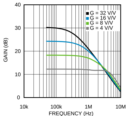
Figure 28. PGA2 Small Signal Bandwidth
