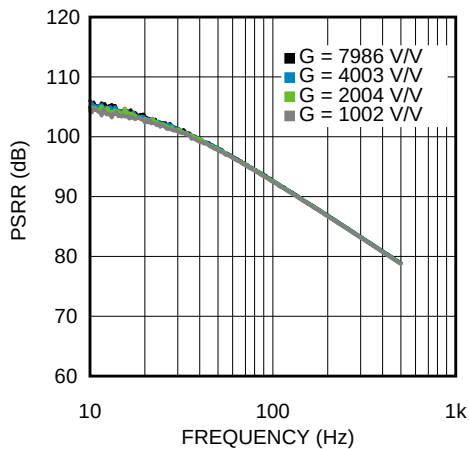
Figure 29. Power Supply Rejection Ratio vs. Frequency
