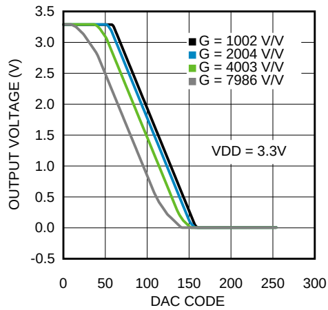
Figure 31. DAC DC Sweep With V_{DD} = 3.3\text{ V}
