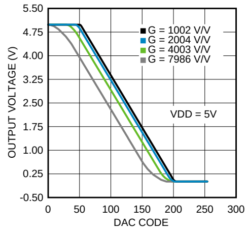
Figure 32. DAC DC Sweep With V_{DD} = 5\text{ V}
