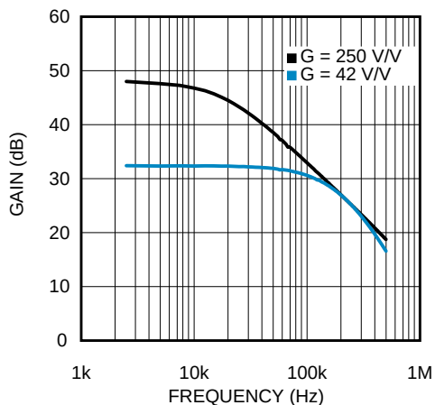
Figure 27. PGA1 Small Signal Bandwidth
