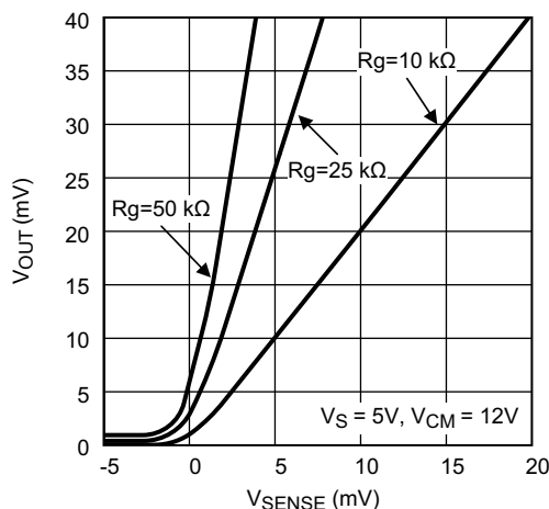
Figure 6-8. Output Voltage vs. V_{\text{SENSE}} (ZOOM Close to 0 V)
