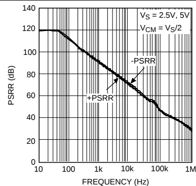
Figure 6. PSRR vs. Frequency
