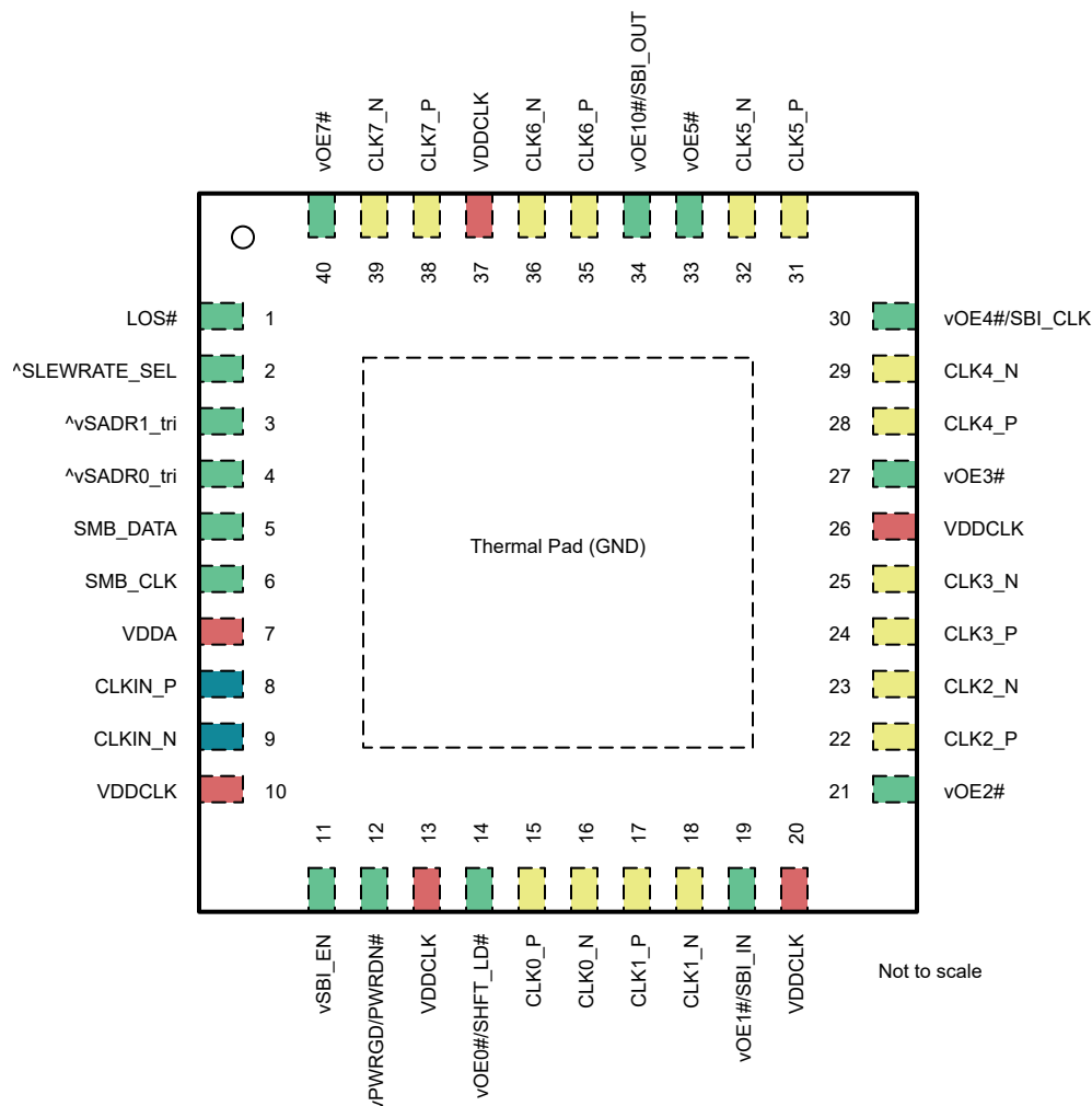
Figure 5-2. LMKDB1108 and LMKDB1108FS 5mm x 5mm VQFN Package 40 Pin Top View
