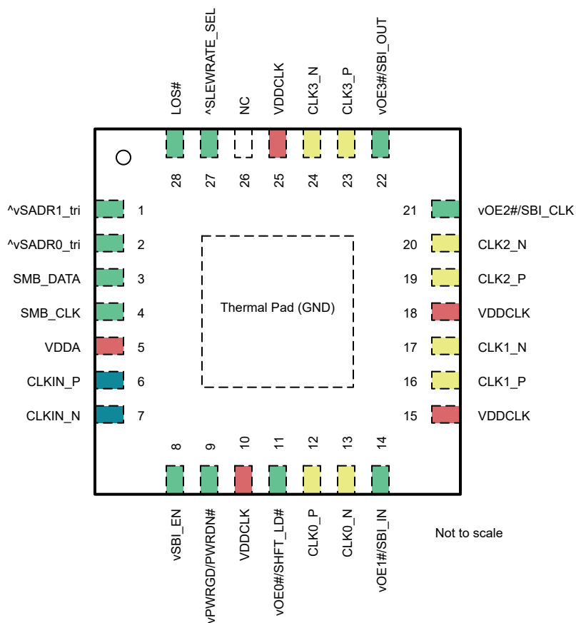
Figure 5-3. LMKDB1104 and LMKDB1104FS 4mm x 4mm VQFN Package 28 Pin Top View
