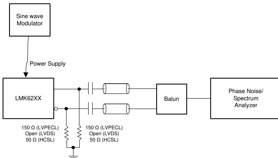
Figure 6-6. HCSL Output AC Configuration During Device Test
