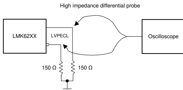
Figure 6-1. LVPECL Output DC Configuration During Device Test
