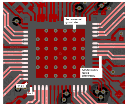
Figure 9-5. PCB Layout Example for LMK5C33216A, Top Layer
