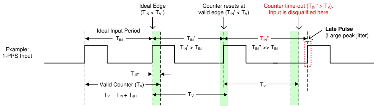
Figure 7-18. 1-PPS Input Window Detector Example
