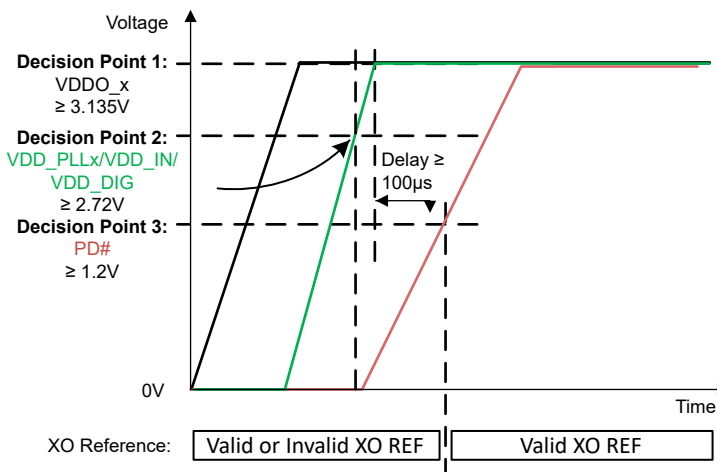
Figure 8-2. Recommendation for Power Up From Split-Supply Rails
