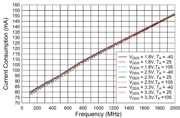
Figure 6-3. LMK1D2104L Current Consumption vs. Frequency, AMP_SELA = 0
