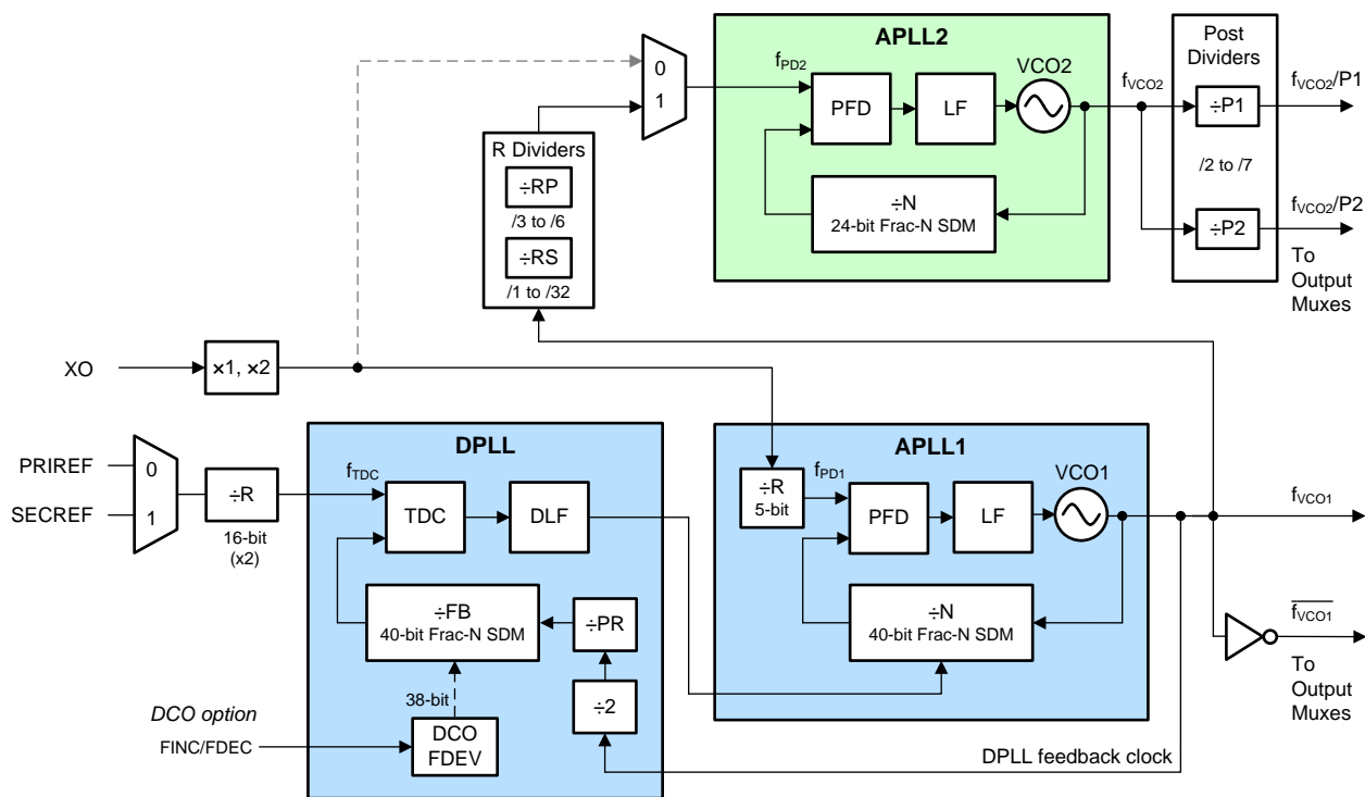
Figure 24. DPLL Mode With Cascaded APLL2
