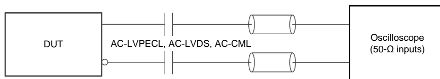
Figure 17. AC-LVPECL, AC-LVDS, AC-CML Output AC Test Configuration
