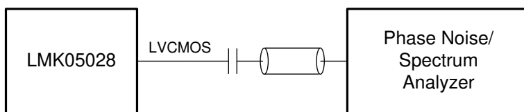
Figure 6-1. LVCMOS Output Test Configuration
