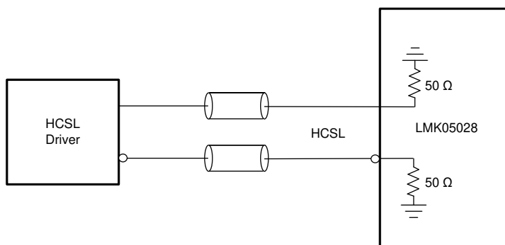
Figure 7-16. DC-Coupled CML (Source Terminated) to Reference (INx) or XO Inputs
