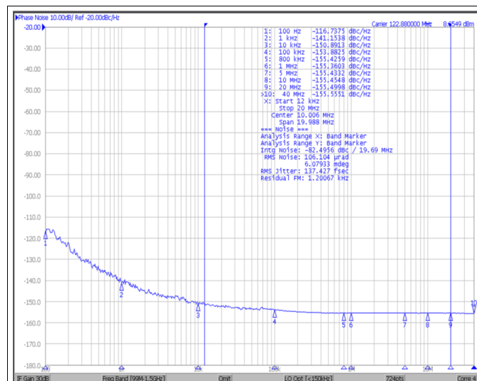
Figure 35. OSCOut, 122.88 MHz, LVC MOS (Norm/Inv) Normal Output Measured, Inverse 50-Ω Termination
