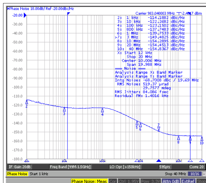
Figure 34. DCLKout4, 983.04-MHz LVPECL16 With 240- \Omega Emitter Resistors CLKout4_5_IDL = 1, CLKout4_5_ODL = 0
