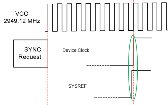
Figure 16. SYSREF to Device Clock Timing Alignment
