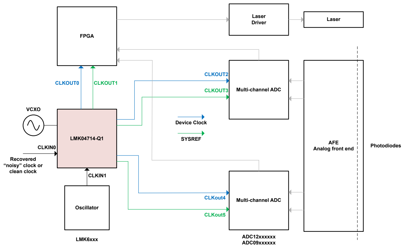
Figure 9-15. Typical LIDAR Automotive Application
