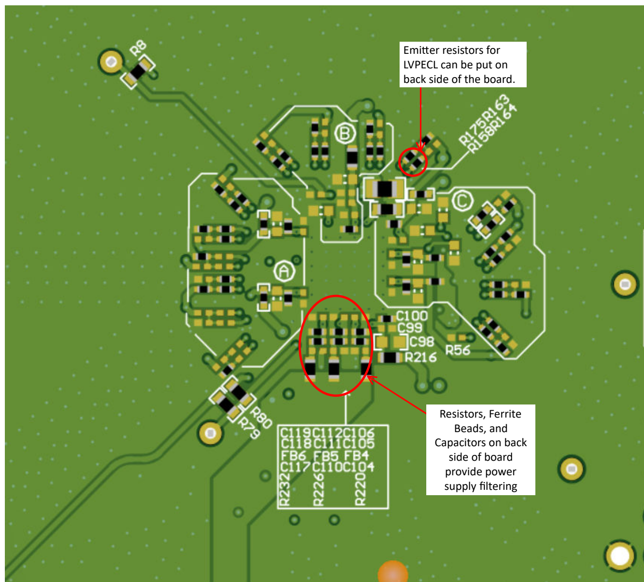
Figure 9-19. Bottom Layer
