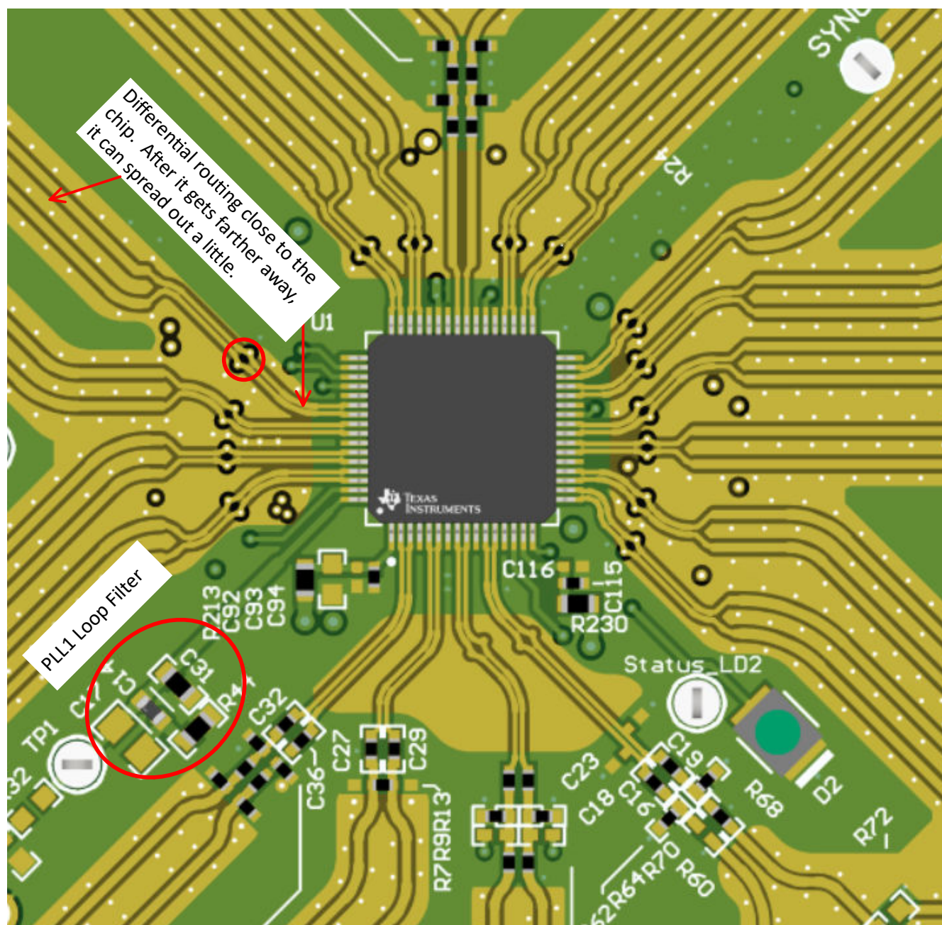
Figure 9-18. Top Layer
