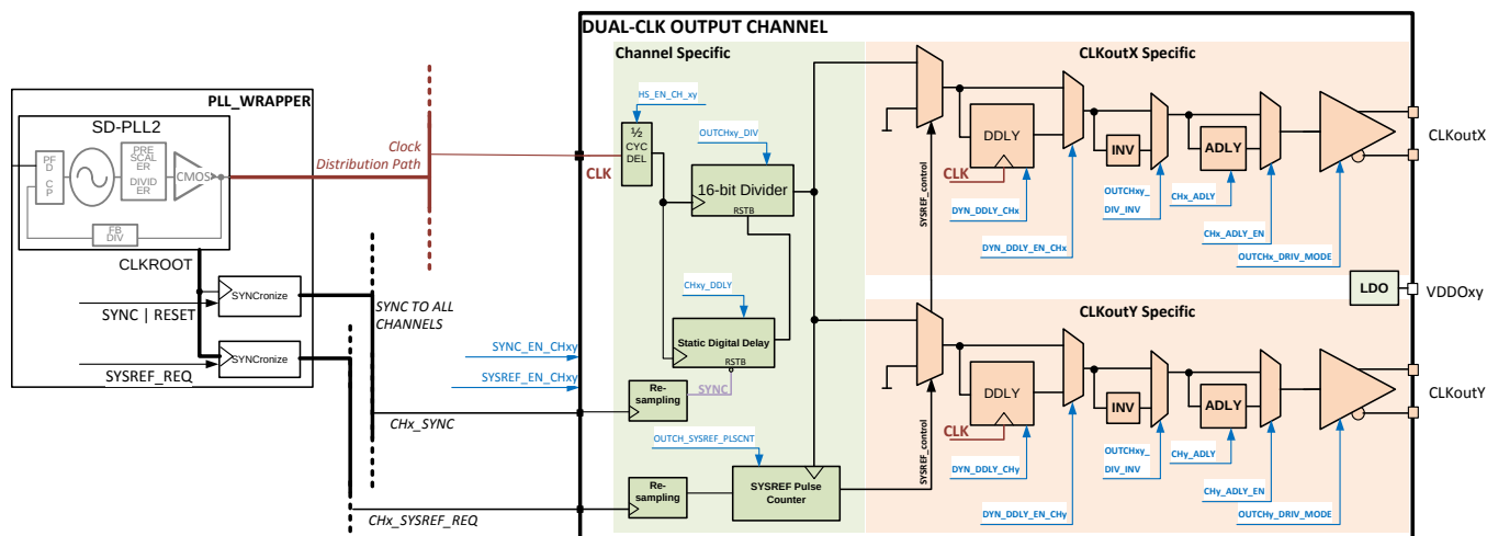
Figure 24. Clock Output Block and SYNC Clcking Path
