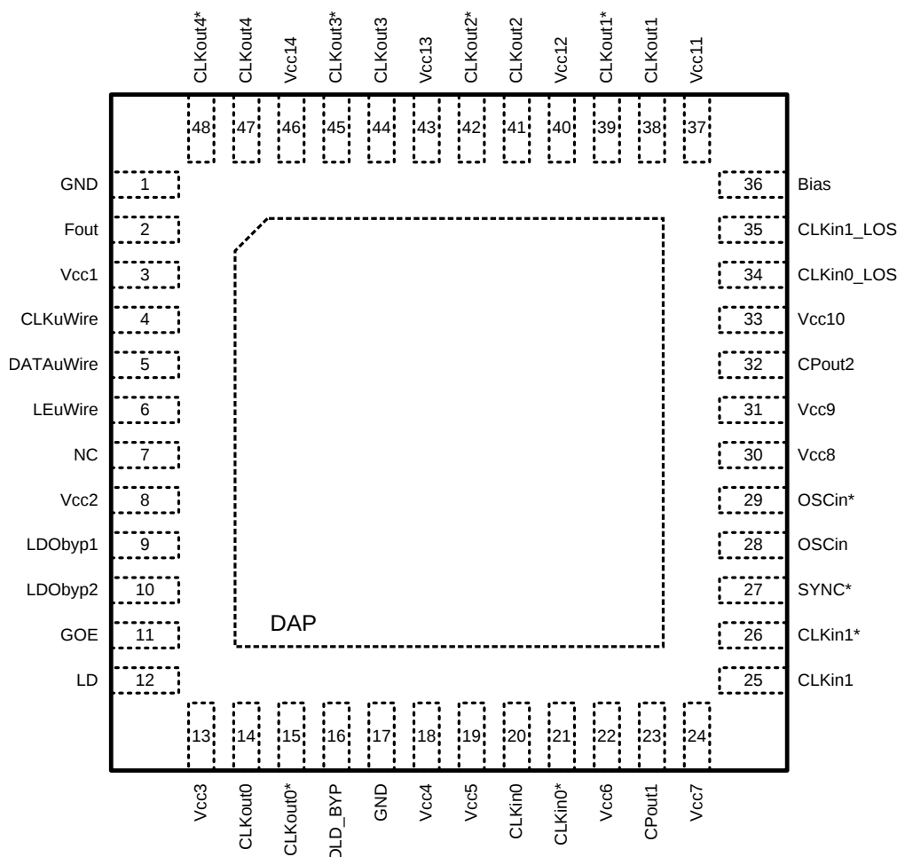
Figure 1. 48-Pin WQFN Package Top Down View
