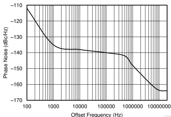
Figure 6-7. Closed-Loop Phase Noise of AC-LVDS Outputs at 161.1328125 MHz With PLL Bandwidth at 400 kHz, Fractional N PLL, 50-MHz Crystal Input, 5-GHz VCO Frequency, Post Divider = 8, Output Divider = 4
