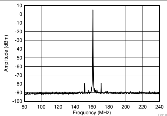
Figure 6-16. 161.1328125 ± 80.56640625-MHz AC-CML Output Spectrum With PLL Bandwidth at 400 kHz, Fractional N PLL, 50-MHz Crystal Input, 5.15625-GHz VCO Frequency, Post Divider = 8, Output Divider = 4
