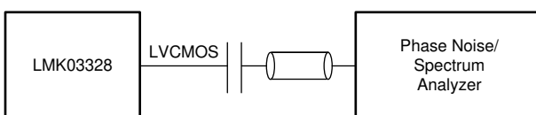
Figure 7-2. LVC MOS Output AC Configuration During Device Test
