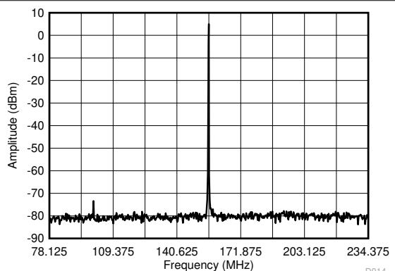
Figure 6-12. 156.25 ± 78.125-MHz AC-CML Output Spectrum With PLL Bandwidth at 1 MHz, Integer N PLL, 50-MHz Crystal Input, 5-GHz VCO Frequency, Post Divider = 8, Output Divider = 4
