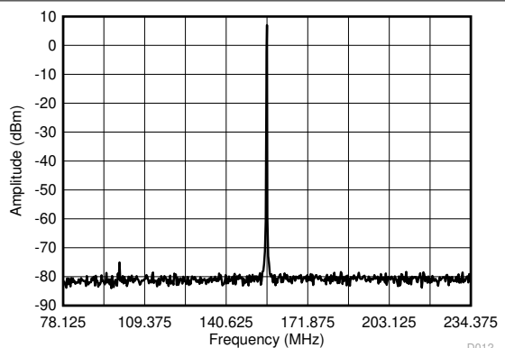
Figure 6-10. 156.25 ± 78.125-MHz AC-LVPECL Output Spectrum With PLL Bandwidth at 1 MHz, Integer N PLL, 50-MHz Crystal Input, 5-GHz VCO Frequency, Post Divider = 8, Output Divider = 4
