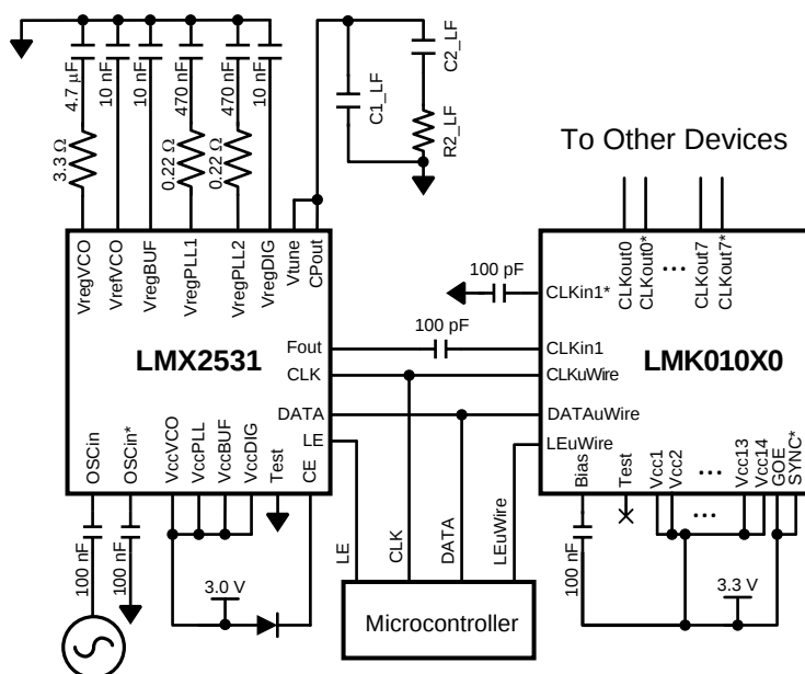
Figure 2. Typical Application
