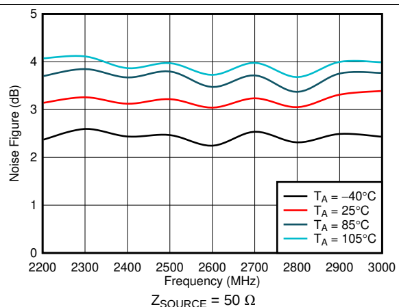
Figure 12. Noise Figure vs Frequency and Temperature
