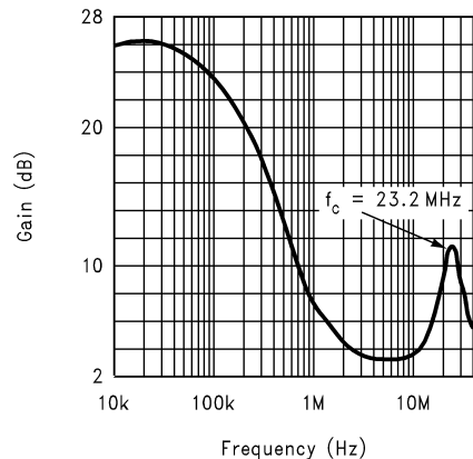
Figure 55. Equalizer Frequency Response
