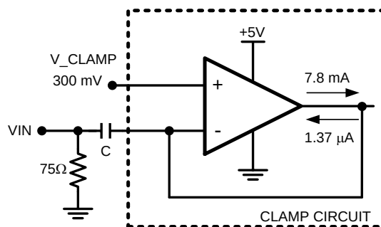
Figure 52. Clamp Circuit
