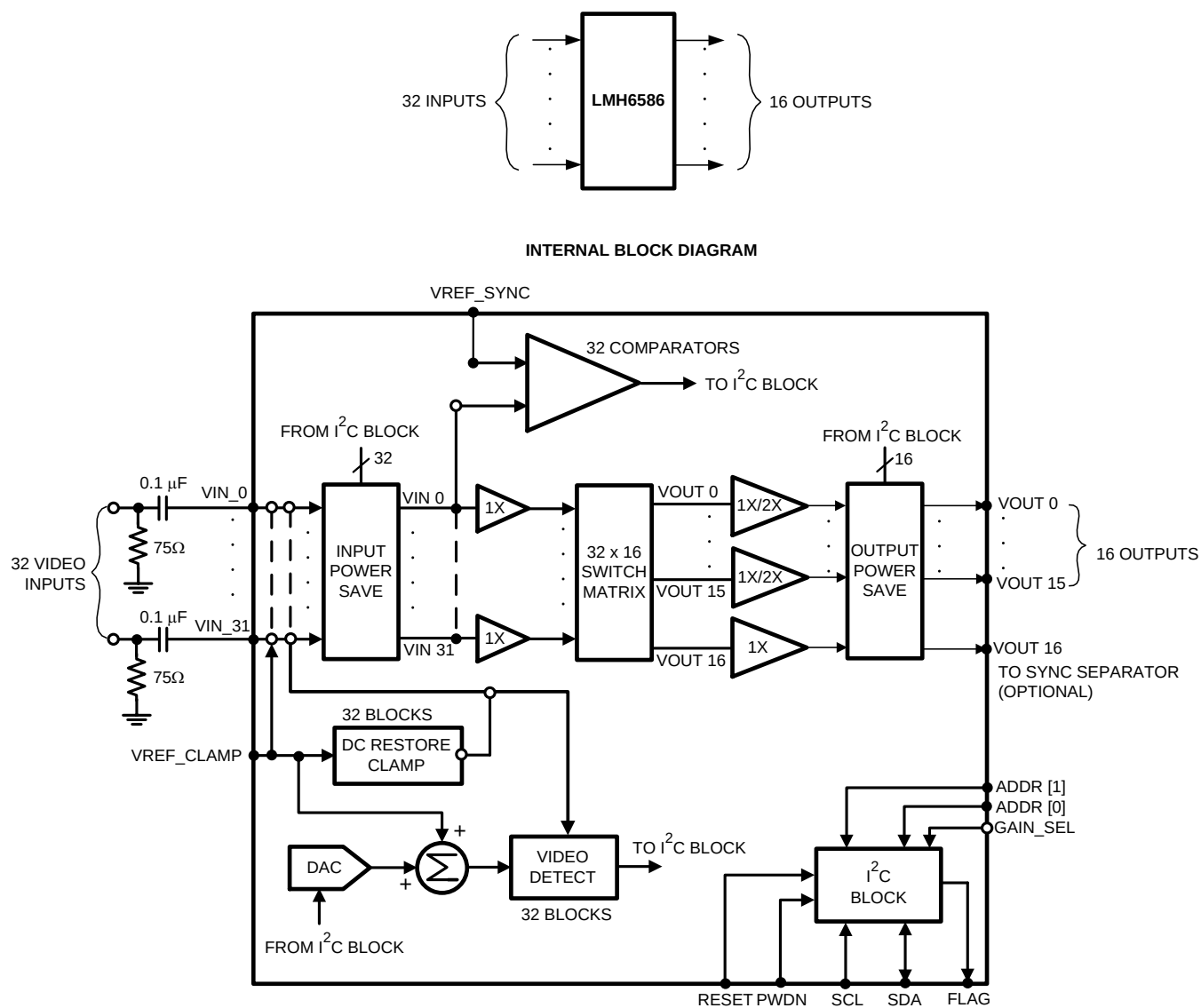
Figure 1. Functional Diagram
