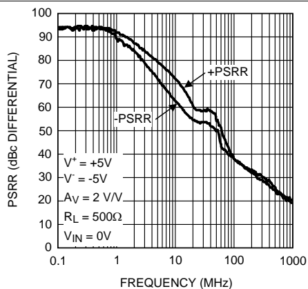
Figure 27. PSRR
