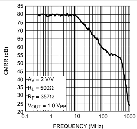
Figure 29. CMRR
