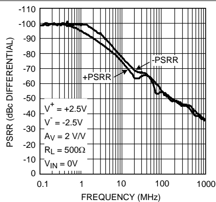
Figure 28. PSRR
