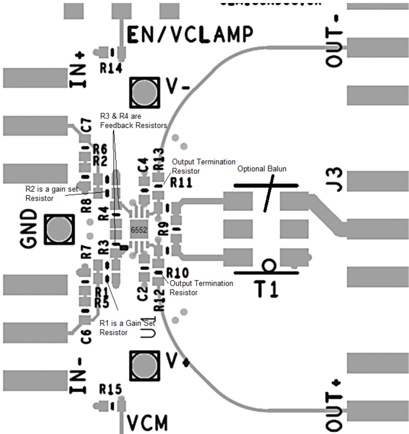
Figure 55. Layout Schematic
