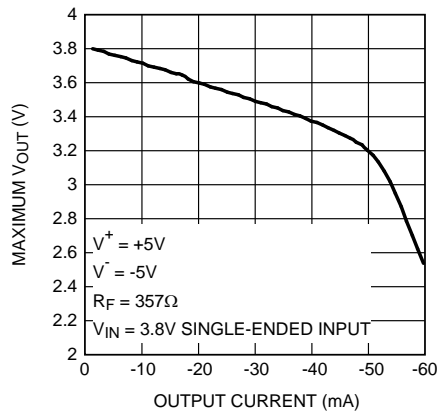
Figure 19. Maximum V_{OUT} vs I_{OUT}
