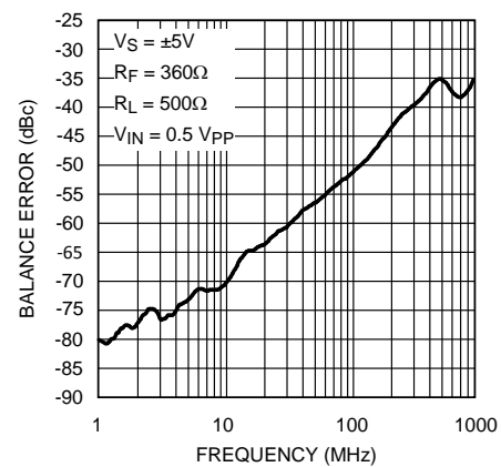
Figure 22. Balance Error
