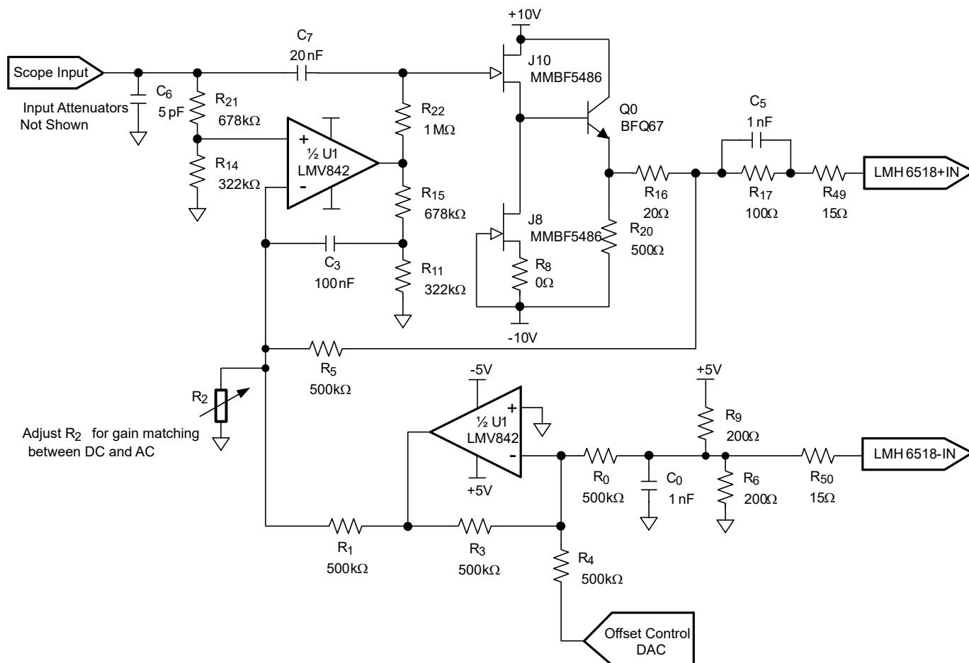
Figure 7-11. JFET LNA Implementation
