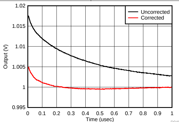
Figure 63. Long-Term Settling Response using Thermal Feedback (Gain = 10, Frequency = 9)
