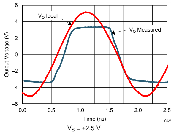
Figure 49. Overdrive Recovery
