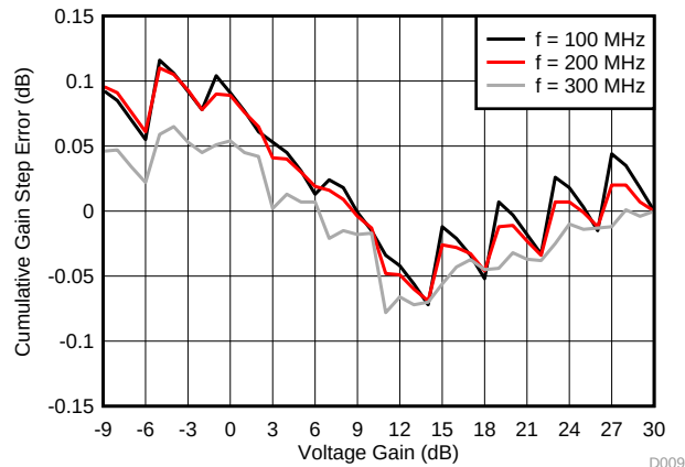
Figure 31. Cumulative Gain Step Error vs Voltage Gain
