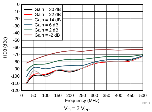
Figure 16. HD3 vs Frequency and Gain Settings
