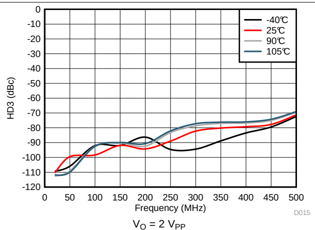
Figure 18. HD3 vs Frequency and Temperature
