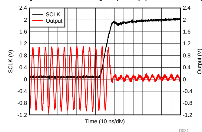
Figure 37. Gain Switching Response ( A_V = 30\text{ dB} to 14\text{ dB} )
