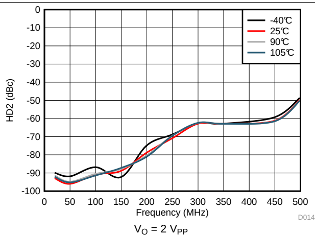
Figure 17. HD2 vs Frequency and Temperature
