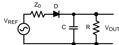
Figure 43. Diode Detector
