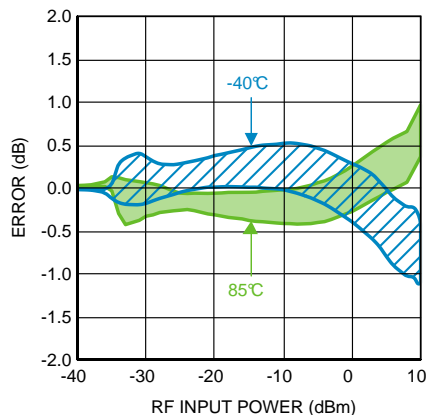
Figure 27. Temperature Variation (50 Units) vs. RF Input Power at 1900 MHz
