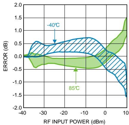
Figure 19. Temperature Variation (50 Units) vs. RF Input Power at 900 MHz
