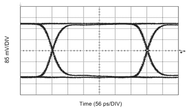
Figure 6. 2.97 Gbps, IN0: 200 m Belden 1694A
