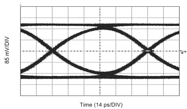
Figure 4. 11.88 Gbps, IN0: 75 m Belden 1694A
