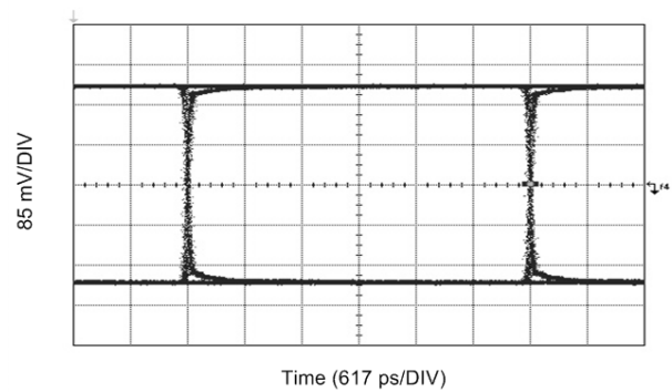
Figure 8. 270 Mbps, IN0: 600 m Belden 1694A
