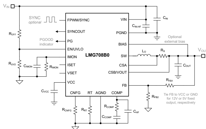
Typical Schematic
