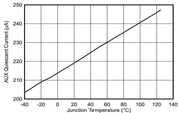
Figure 5-5. AUX Quiescent Current vs Junction Temperature
