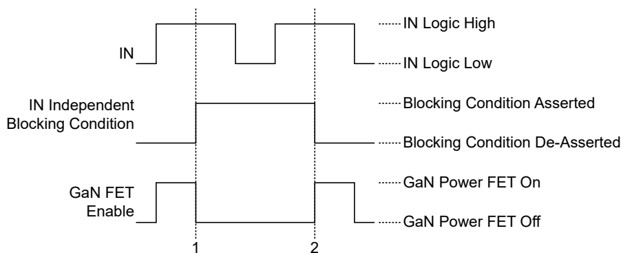
Figure 7-4. IN Independent Blocking Condition Operation
