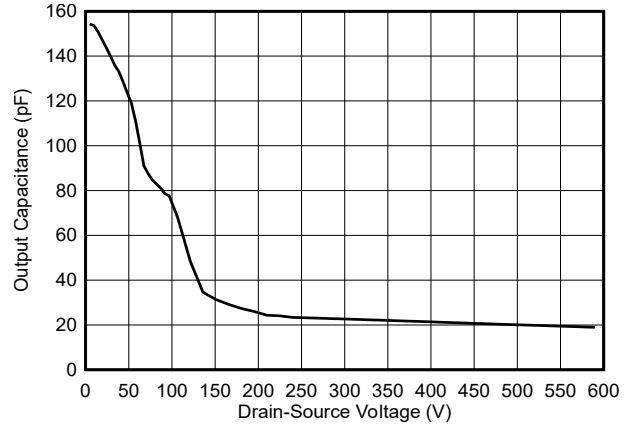
Figure 5-2. Output Capacitance vs Drain-Source Voltage
