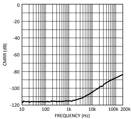
Figure 87. Cmr vs Frequency V_{CC} = 17V , V_{EE} = -17V R_L = 600\Omega
