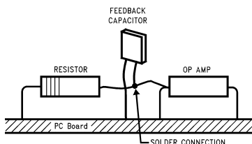
Figure 6-10. Air Wiring
