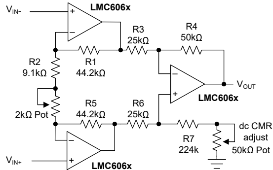
Figure 6-4. Instrumentation Amplifier
