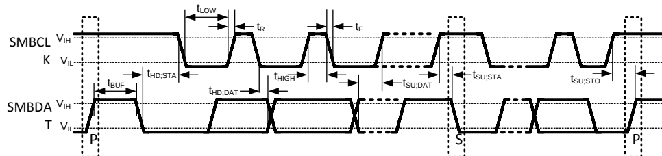
Figure 1. SMBus Communication
