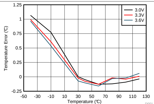
Figure 7. Remote 2 Temperature Error, T_A = T_D
