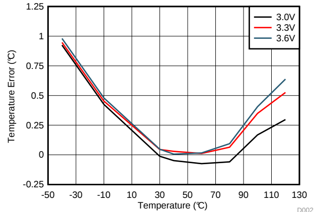
Figure 5. Local Temperature Error, T_A = T_D
