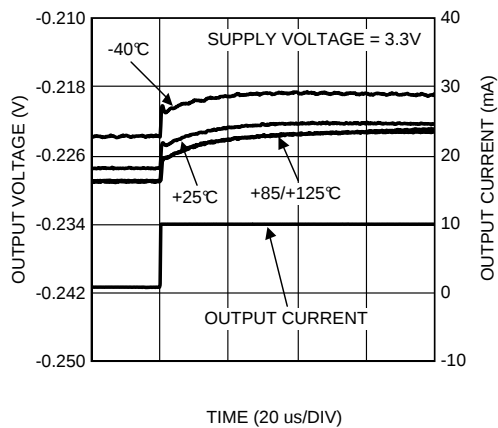
Figure 15. Transient Response
