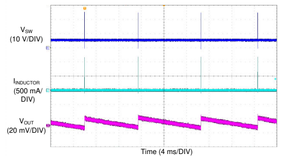
Figure 8-7. LM76005-Q1 Frequency Dropout
