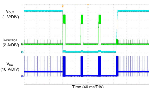
Figure 8-23. LM76005-Q1 Start-up With Pre-Biased Output
