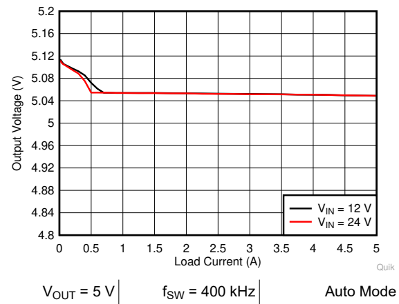
Figure 8-5. LM76005-Q1 Load and Line Regulation
