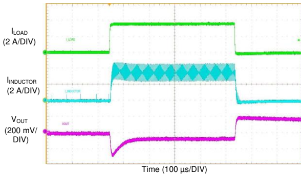
Figure 73. LM76003-Q1 Load Transient
