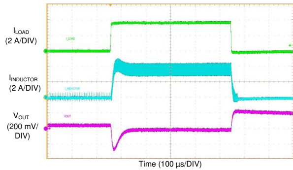
Figure 77. LM76003-Q1 Load Transient
