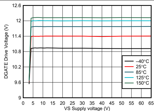
Figure 6-8. DGATE Drive Voltage vs Supply Voltage
