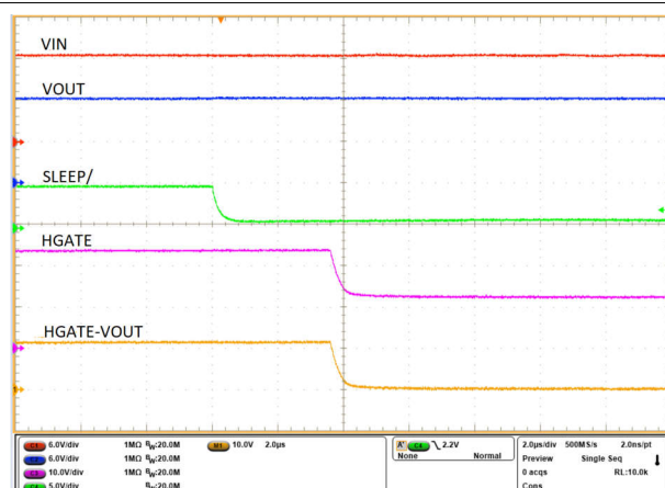
Figure 9-19. SLEEP Mode Entry (SLEEP = Low, EN = High)
