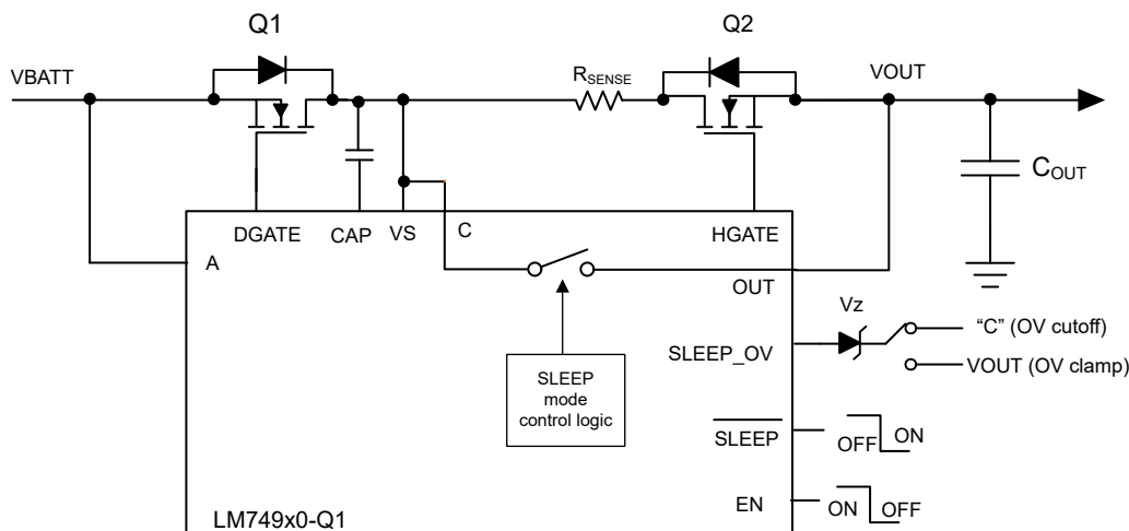
Figure 8-11. Increasing SLEEP_OV Threshold Using an External Zener Diode
