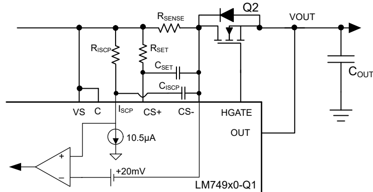
Figure 8-7. Short Circuit Protection With Deglitch Filter
