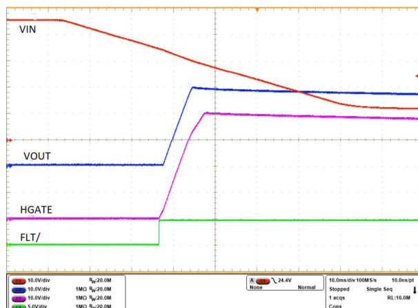
Figure 9-15. Overvoltage Recovery
