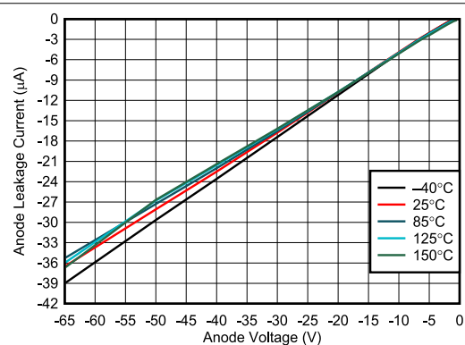
Figure 6-10. ANODE Leakage Current vs Reverse ANODE Voltage
