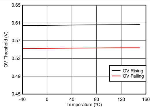
Figure 6-12. OVP Thresholds vs Temperature
