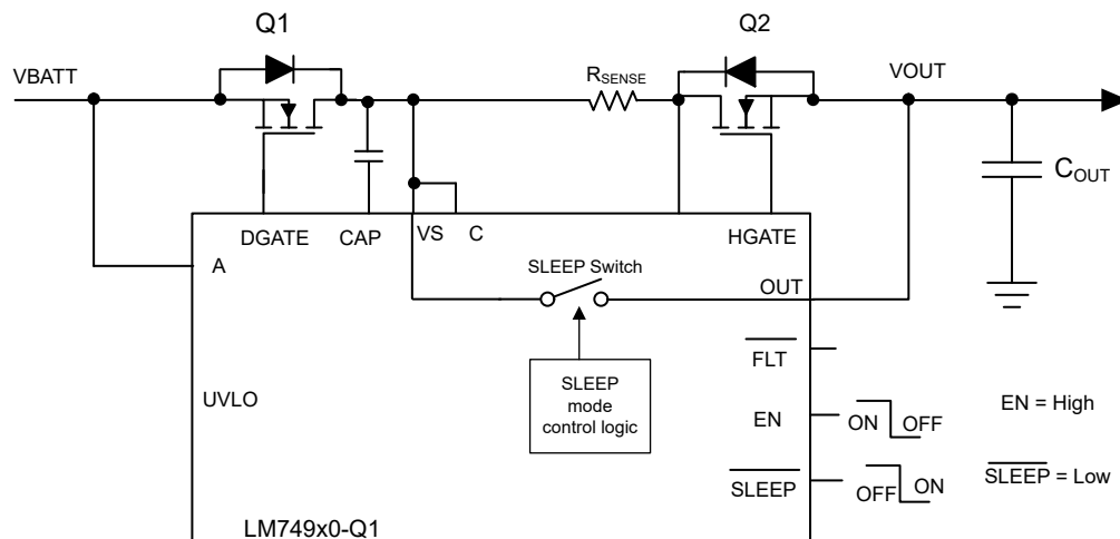
Figure 8-10. LM749x0-Q1 SLEEP Mode Operation
