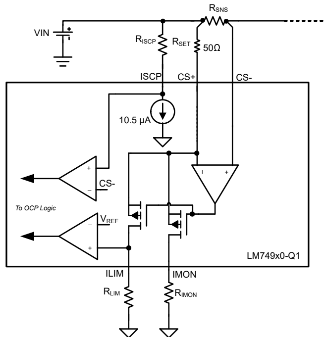
Figure 8-8. Analog Current Monitoring
