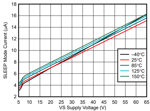
Figure 6-3. SLEEP Mode Current vs Supply Voltage
