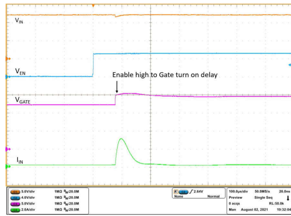
Figure 9-11. Enable Turn ON Delay
