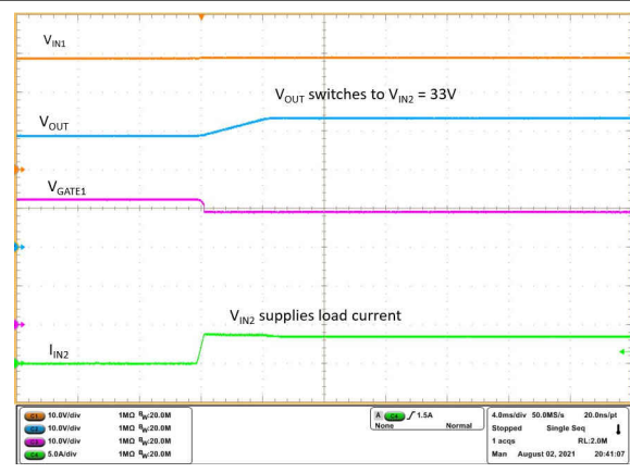
Figure 9-13. ORing V_{IN1} to V_{IN2} Switch Over
