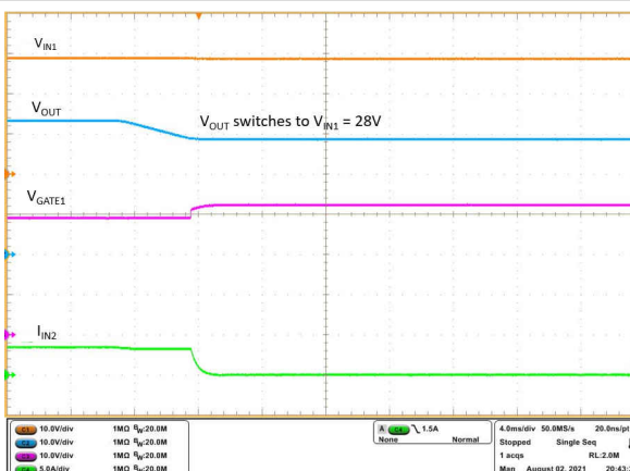
Figure 9-15. ORing V_{IN2} to V_{IN1} Switch Over
