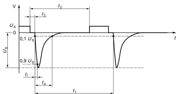
Figure 10-3. ISO 7637-2 Pulse 1
