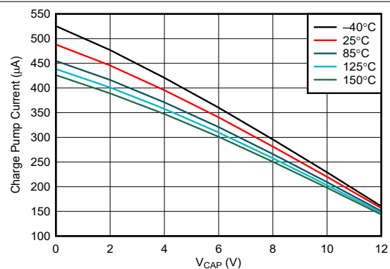
Figure 7-4. Charge Pump V-I Characteristics at V_S \geq 12 V
