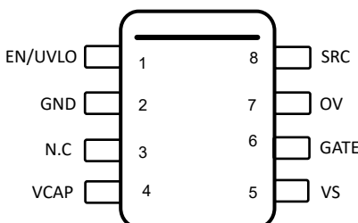
Figure 6-1. DDF Package 8-Pin SOT-23 LM74502-Q1, LM74502H-Q1 Top View
