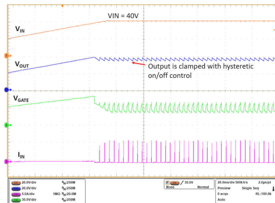
Time (20 ms/DIV) Figure 10-10. Overvoltage Clamp Response
