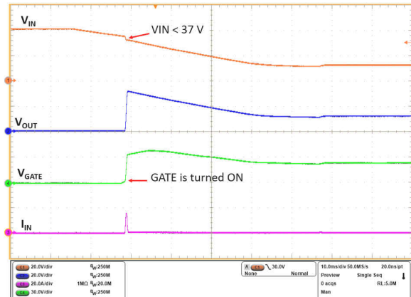
Time (10 ms/DIV) Figure 10-9. Overvoltage Recovery
