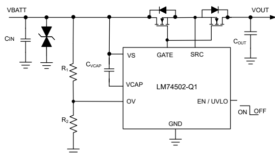
LM74502-Q1 Typical Application Schematic
