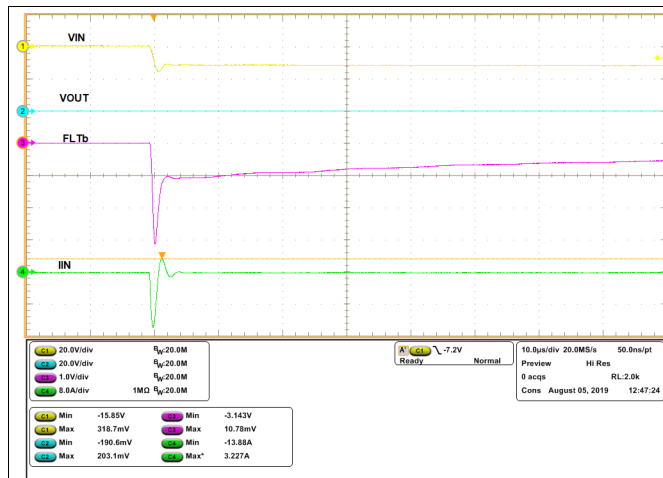
Figure 44. Protection from Reverse Battery [ V_{IN} = -12 V, V_{OUT} = 0 V, I_{LIM} = 2.23 A ]
