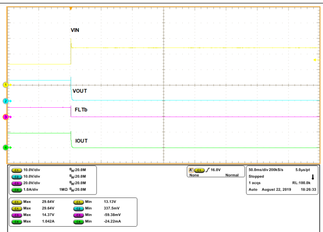
Figure 45. Protection from overvoltage at Input [ V_{IN} = 36 V, R_{LOAD} = 14 \Omega , I_{LIM} = 2.23 A ]
