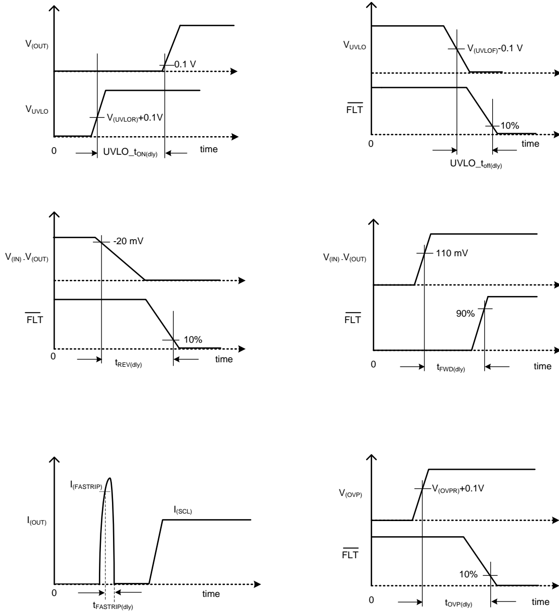
Figure 19. Timing Waveforms
