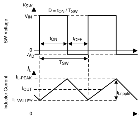
Figure 8-3. SW Voltage and Inductor Current Waveforms in CCM
