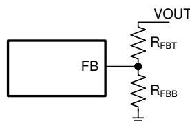
Figure 8-4. Output Voltage Setting by Resistor Divider
