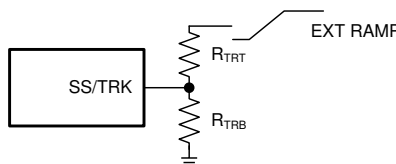
Figure 8-9. Soft-start Tracking External Ramp
