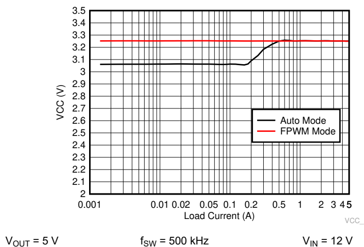
Figure 8-8. VCC Voltage versus Load Current
