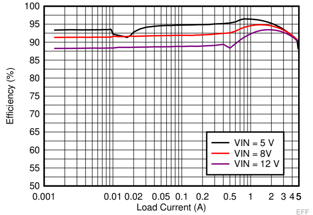
Figure 9-9. LM73605-Q1 Efficiency
