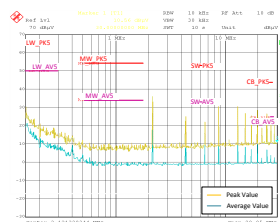
Figure 9-63. LM73606-Q1 Conducted EMI Result versus CISPR25 Limits - Low Frequency
