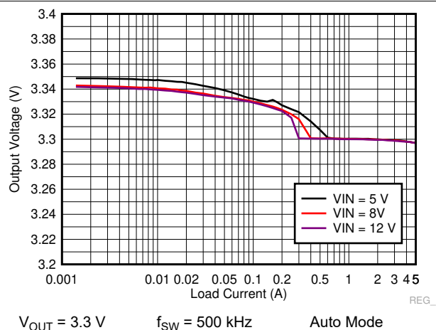
Figure 9-31. LM73605-Q1 Load and Line Regulation
