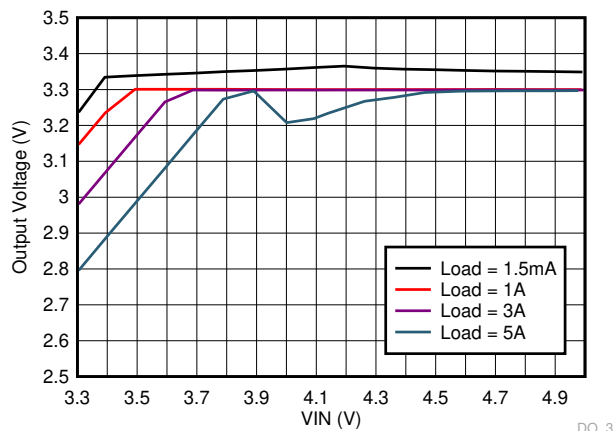
Figure 9-41. LM73606-Q1 Dropout Curve
