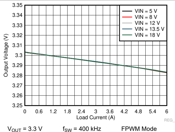
Figure 9-28. LM73606-Q1 Load and Line Regulation
