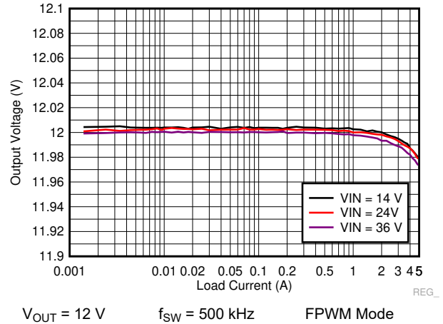
Figure 9-34. LM73605-Q1 Load and Line Regulation
