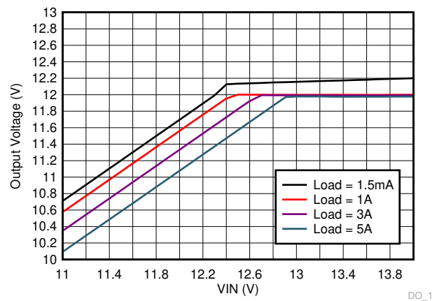
Figure 9-42. LM73606-Q1 Dropout Curve
