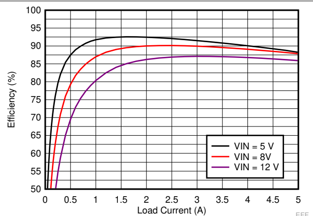
Figure 9-6. LM73605-Q1 Efficiency
