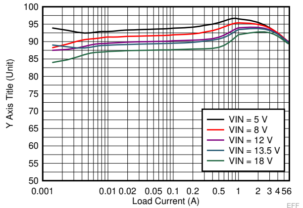
Figure 9-3. LM73606-Q1 Efficiency
