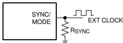
Figure 8-13. Frequency Synchronization
