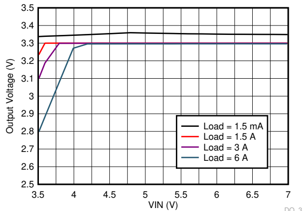
Figure 9-39. LM73605-Q1 Dropout Curve
