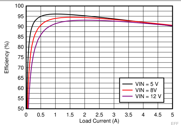
Figure 9-4. LM73606-Q1 Efficiency
