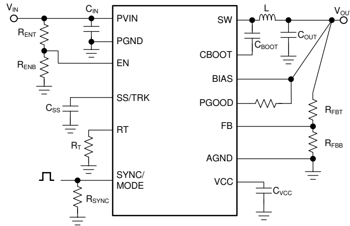
Figure 9-2. LM73605-Q1/6-Q1 Comprehensive Schematic with All Features Utilized
