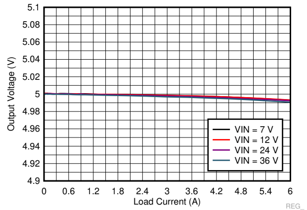
Figure 9-22. LM73606-Q1 Load and Line Regulation
