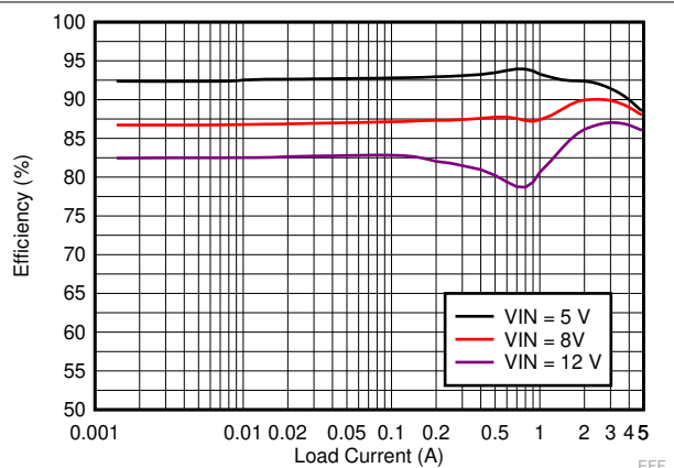
Figure 9-5. LM73605-Q1 Efficiency
