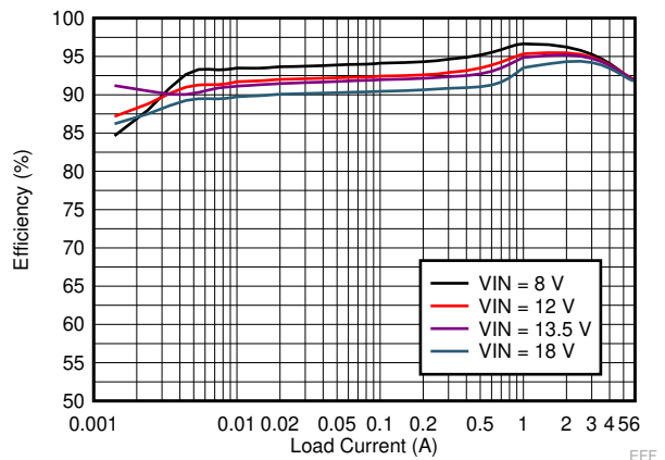
Figure 9-9. LM73605-Q1 Efficiency
