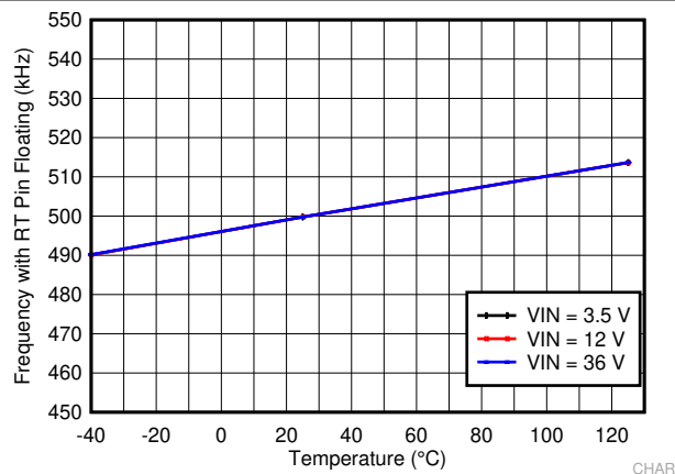
Figure 7-7. Switching Frequency with RT Pin Open Circuit
