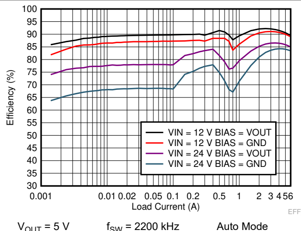
Figure 8-6. LM73606-Q1 Efficiency Comparison With Bias = V_{OUT} to Bias = GND in Auto Mode
