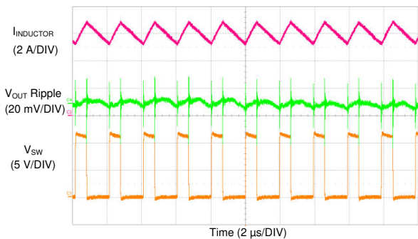
Figure 9-47. LM73606-Q1 Switching Waveform and V_{OUT} Ripple
