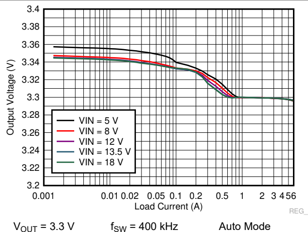
Figure 9-27. LM73606-Q1 Load and Line Regulation
