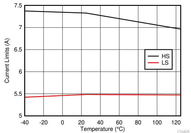
Figure 7-4. LM73605-Q1 High-Side and Low-Side Current Limits
