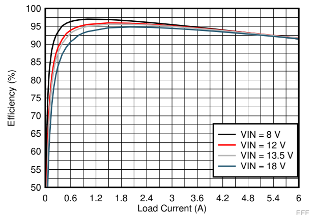
Figure 9-10. LM73605-Q1 Efficiency
