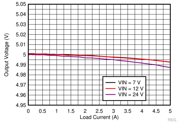
Figure 9-24. LM73606-Q1 Load and Line Regulation
