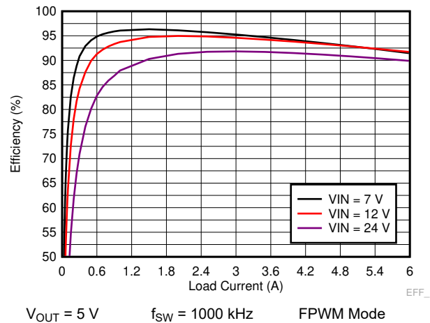
Figure 9-16. LM73606-Q1 Efficiency
