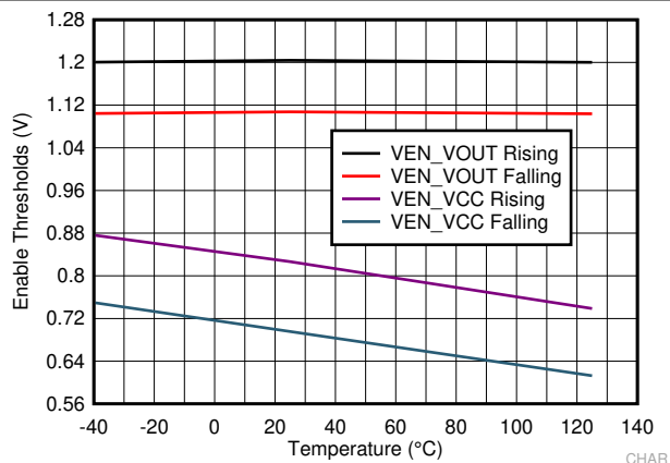
Figure 7-8. Enable Thresholds
