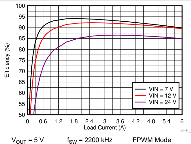
Figure 9-18. LM73606-Q1 Efficiency
