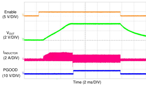
Figure 9-51. LM73606-Q1 Overcurrent Behavior
