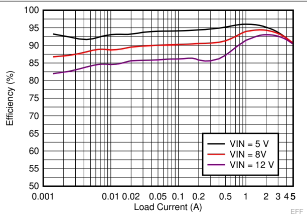
Figure 9-3. LM73606-Q1 Efficiency
