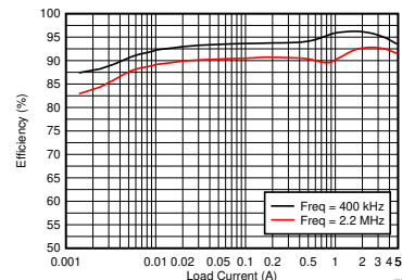
Efficiency versus Load Current V_{\text{OUT}} = 5 \text{ V} , V_{\text{IN}} = 12 \text{ V} , Auto Mode
