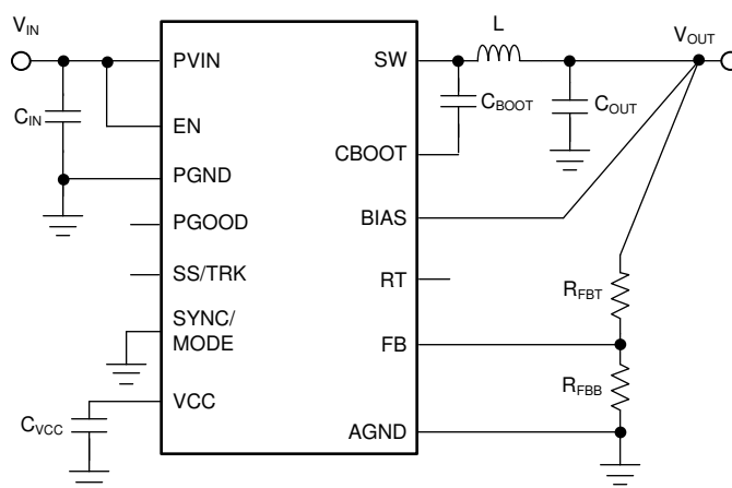
Figure 9-1. LM73605-Q1/6-Q1 Basic Schematic
