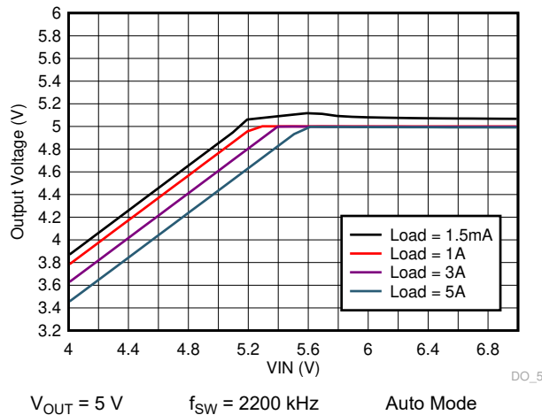
Figure 9-37. LM73605-Q1 Dropout Curve
