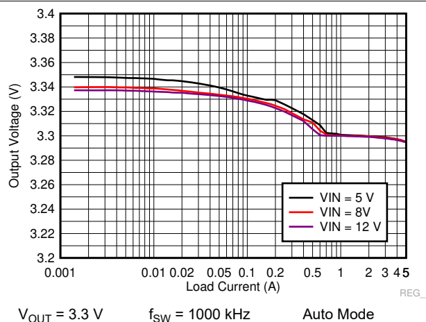
Figure 9-32. LM73605-Q1 Load and Line Regulation
