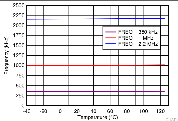
Figure 7-6. Switching Frequency Set by R_T Resistor
