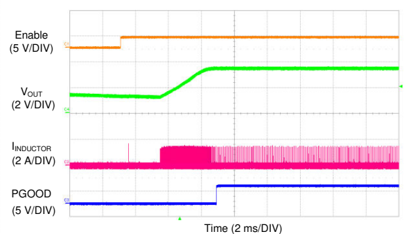
Figure 9-54. LM73606-Q1 Soft Start With 200-mA Load in Auto Mode
