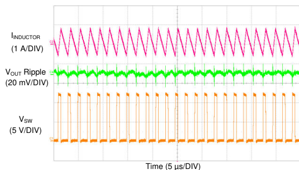
Figure 9-46. LM73606-Q1 Switching Waveform and V_{OUT} Ripple
