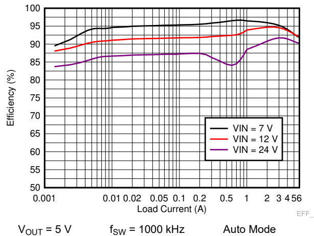
Figure 9-15. LM73606-Q1 Efficiency
