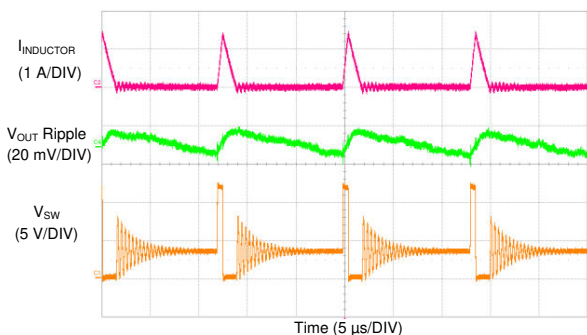
Figure 9-45. LM73606-Q1 Switching Waveform and V_{OUT} Ripple
