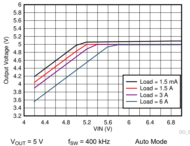
Figure 9-35. LM73606-Q1 Dropout Curve
