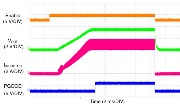
Figure 9-53. LM73606-Q1 Soft Start With 200-mA Load in FPWM Mode
