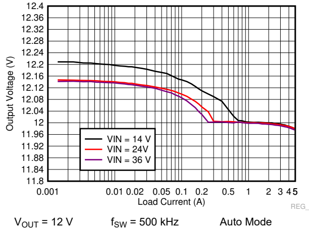
Figure 9-33. LM73605-Q1 Load and Line Regulation
