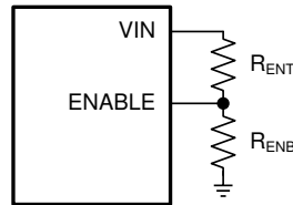
Figure 8-5. System UVLO
