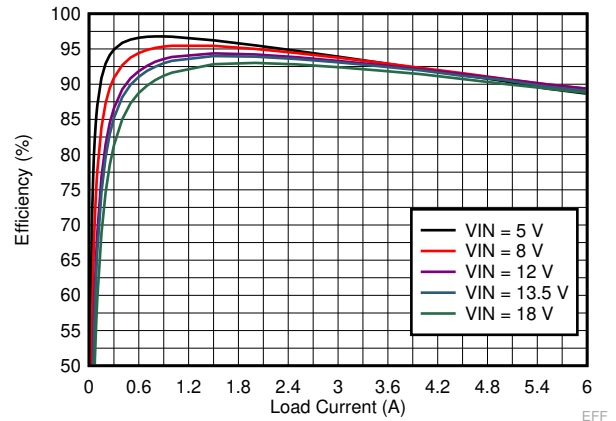
Figure 9-4. LM73606-Q1 Efficiency
