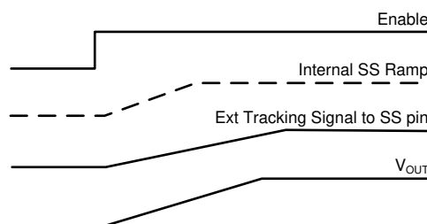
Figure 8-10. Tracking With Longer Start-up Time Than the Internal Ramp
