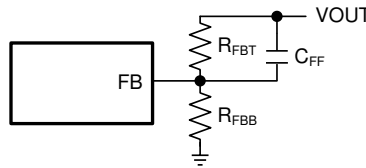
Figure 8-14. Feedforward Capacitor for Loop Compensation
