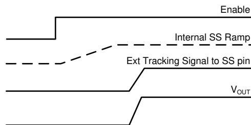
Figure 8-11. Tracking With Shorter Start-up Time Than the Internal Ramp
