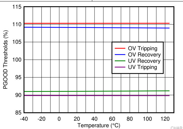
Figure 7-9. PGOOD Thresholds
