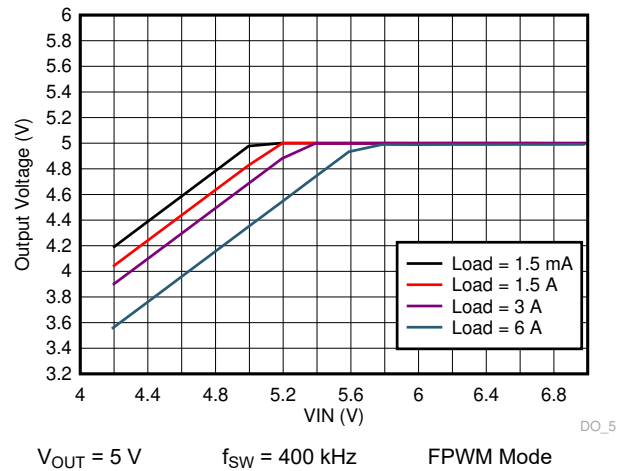
Figure 9-36. LM73606-Q1 Dropout Curve
