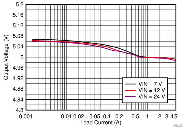
Figure 9-23. LM73606-Q1 Load and Line Regulation
