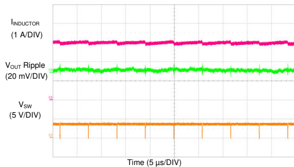
Figure 9-48. LM73606-Q1 Switching Waveform and V_{OUT} Ripple
