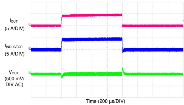
Figure 9-58. LM73606-Q1 Load Transients
