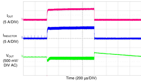
Figure 9-57. LM73606-Q1 Load Transients
