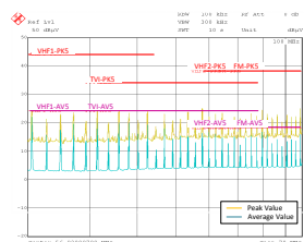
Figure 9-64. LM73606-Q1 Conducted EMI Result versus CISPR25 Limits - High Frequency
