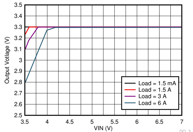
Figure 9-40. LM73605-Q1 Dropout Curve
