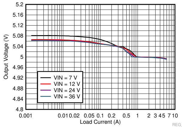
Figure 9-21. LM73606-Q1 Load and Line Regulation
