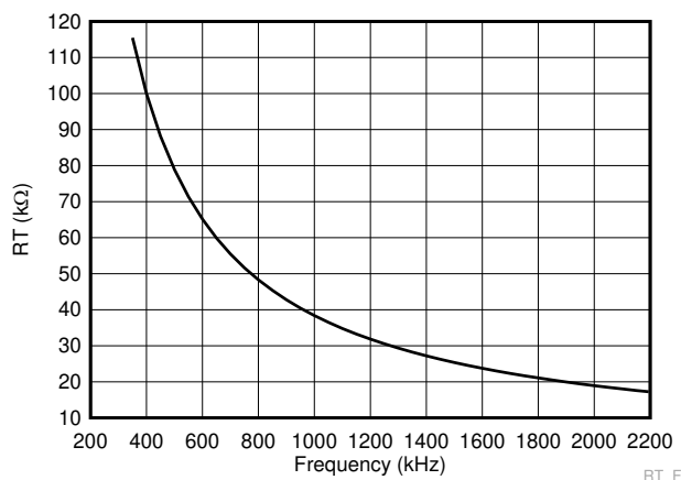
Figure 8-12. R_T Resistance versus Switching Frequency
