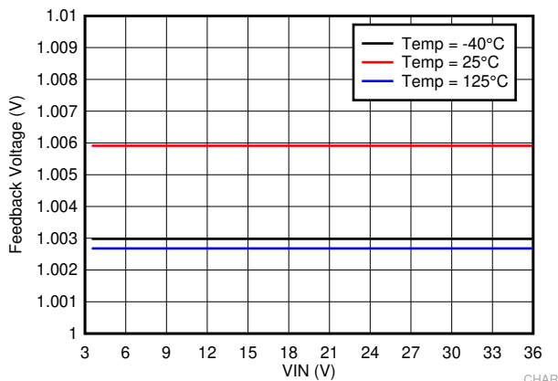
Figure 7-3. Feedback Voltage
