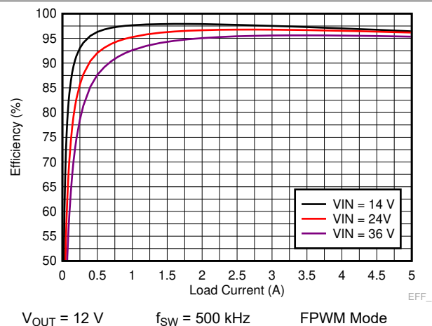
Figure 9-20. LM73605-Q1 Efficiency
