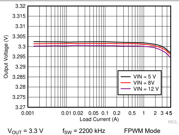
Figure 9-30. LM73605-Q1 Load and Line Regulation
