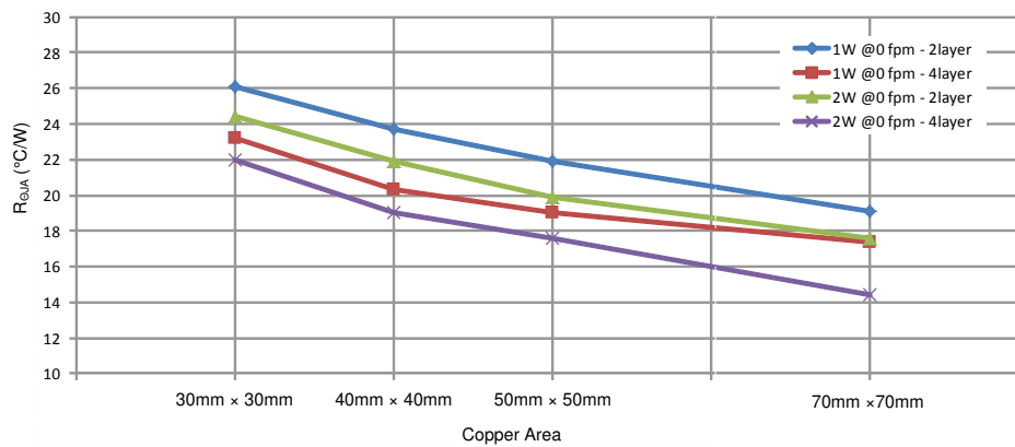
Figure 9-2. Measured R_{\theta JA} versus PCB Copper Area on 2-Layer Boards and 4-Layer Boards
