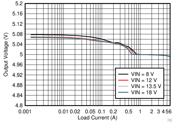
Figure 9-21. LM73606-Q1 Load and Line Regulation
