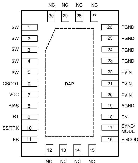
Figure 6-1. RNP Package 30-Pin Wettable Flanks QFN (WQFN) 6 mm × 4 mm × 0.8 mm Top View
