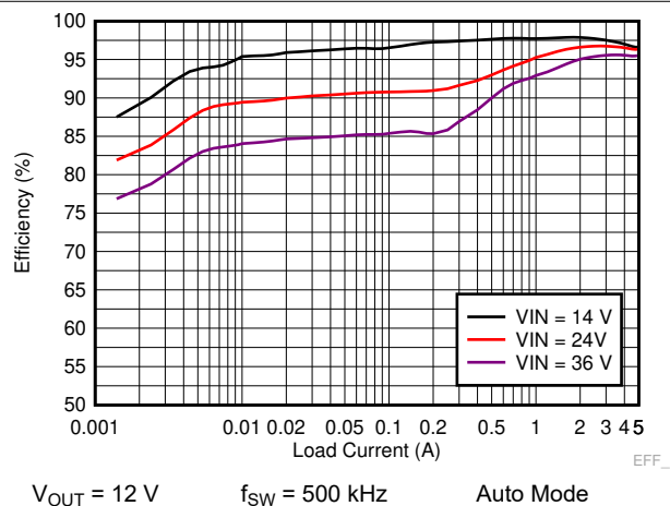
Figure 9-19. LM73605-Q1 Efficiency
