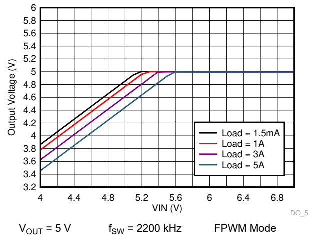
Figure 9-38. LM73605-Q1 Dropout Curve
