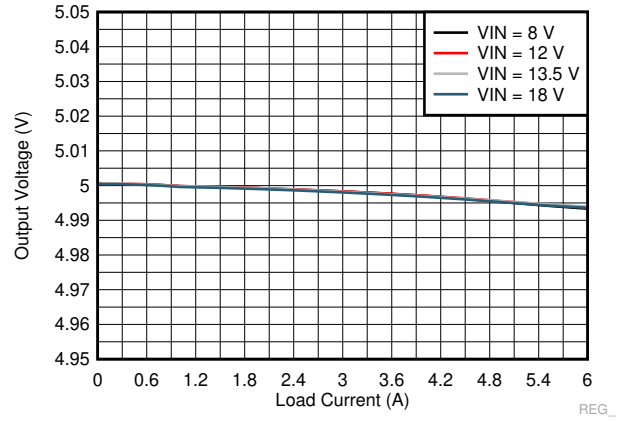
Figure 9-22. LM73606-Q1 Load and Line Regulation
