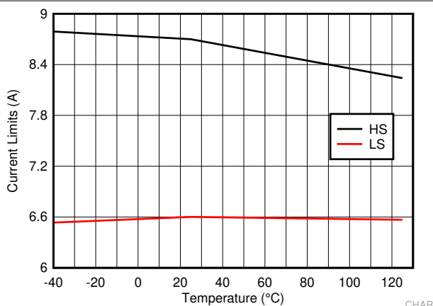
Figure 7-5. LM73605-Q1 High-Side and Low-Side Current Limit
