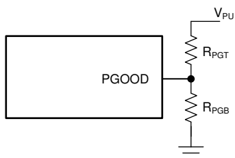
Figure 8-15. Divider for PGOOD Pullup Voltage
