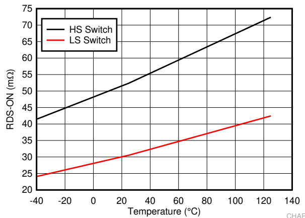
Figure 7-1. High-Side and Low-Side Switches R_{DS-ON}
