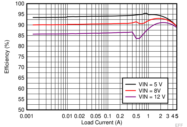
Figure 9-10. LM73605-Q1 Efficiency
