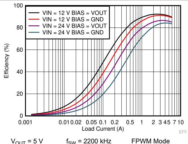
Figure 8-7. LM73606-Q1 Efficiency Comparison With Bias = V_{OUT} to Bias = GND in FPWM Mode
