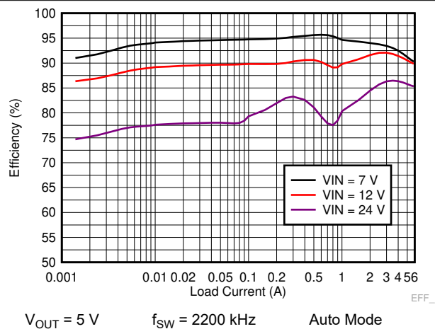
Figure 9-17. LM73606-Q1 Efficiency
