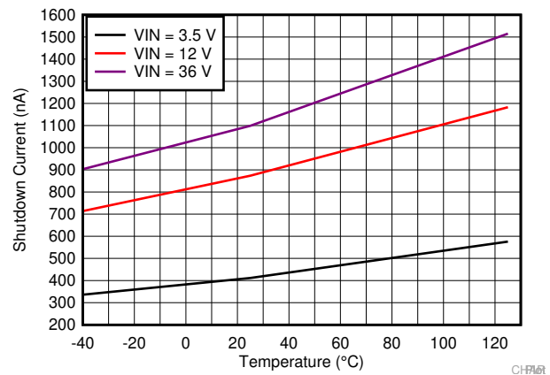
Figure 7-2. Shutdown Quiescent Current
