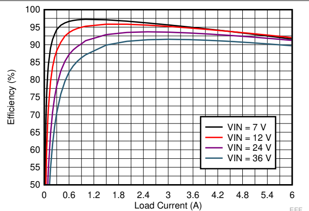
Figure 9-12. LM73606-Q1 Efficiency
