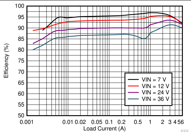
Figure 9-11. LM73606-Q1 Efficiency
