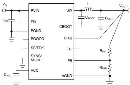
Simplified Schematic
