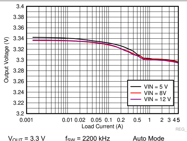
Figure 9-29. LM73605-Q1 Load and Line Regulation
