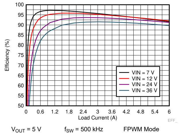
Figure 9-14. LM73606-Q1 Efficiency
