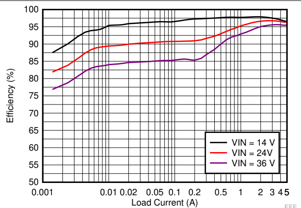
Figure 9-17. LM73606-Q1 Efficiency
