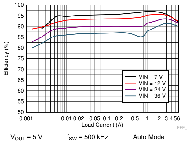
Figure 9-13. LM73606-Q1 Efficiency
