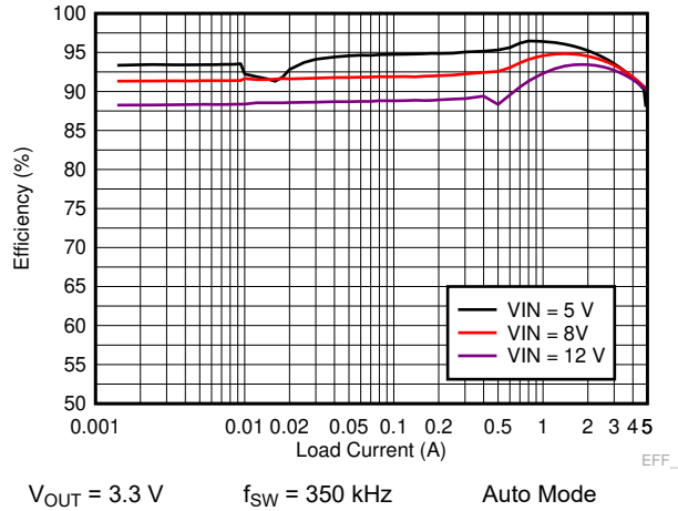
Figure 9-9. LM73605-Q1 Efficiency
