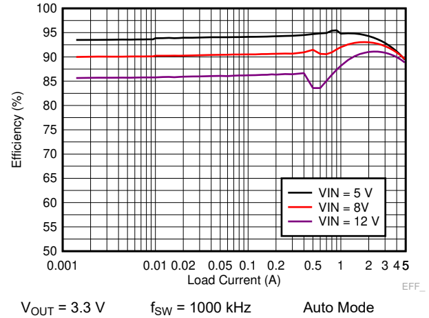
Figure 9-10. LM73605-Q1 Efficiency
