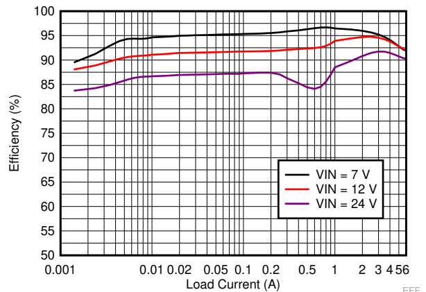
Figure 9-15. LM73606-Q1 Efficiency
