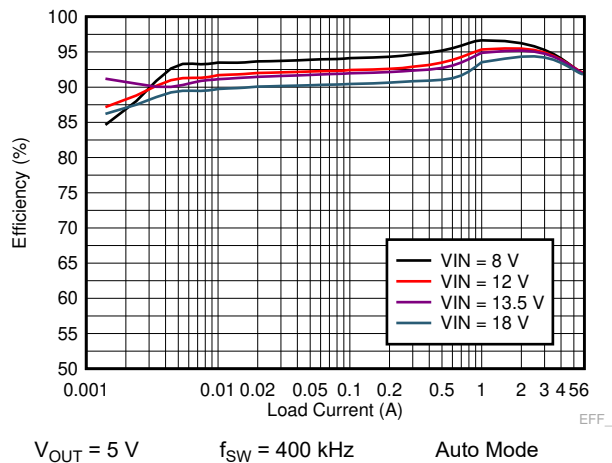
Figure 9-11. LM73606-Q1 Efficiency
