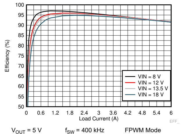
Figure 9-12. LM73606-Q1 Efficiency
