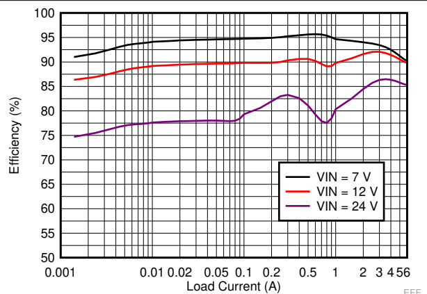
Figure 9-15. LM73606-Q1 Efficiency
