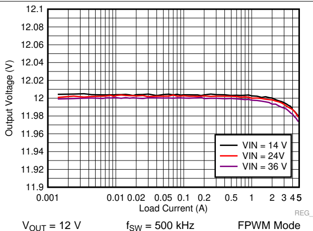
Figure 50. LM73605 Load and Line Regulation
