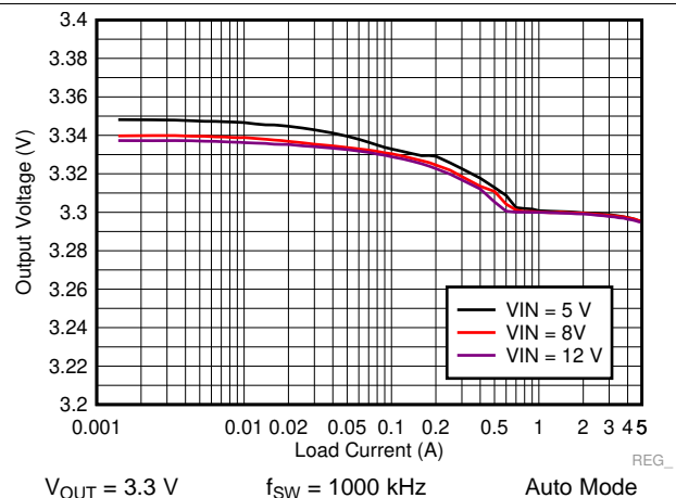
Figure 48. LM73605 Load and Line Regulation
