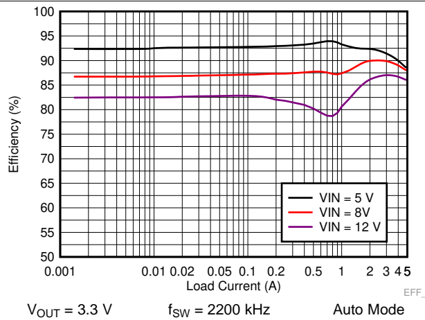
Figure 29. LM73605 Efficiency
