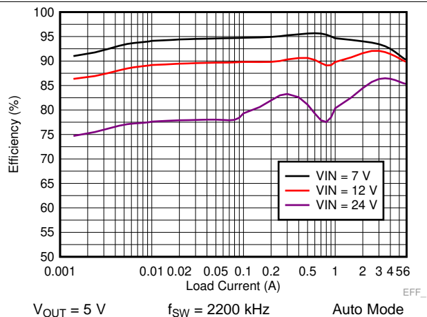
Figure 37. LM73606 Efficiency
