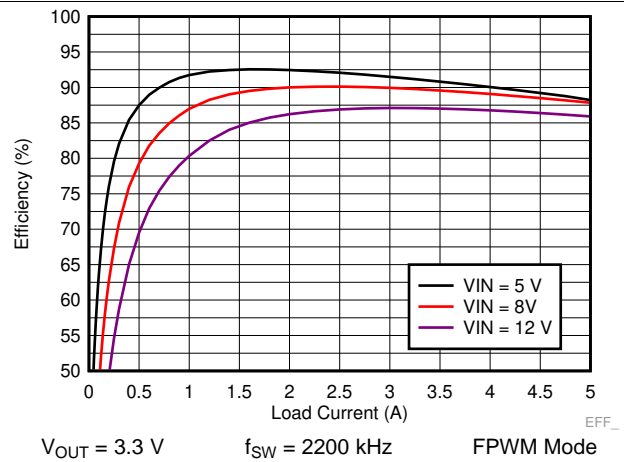
Figure 30. LM73605 Efficiency
