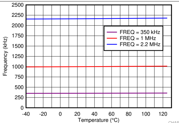
Figure 6. Switching Frequency Set by R_T Resistor
