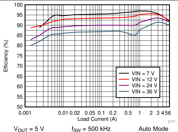
Figure 33. LM73606 Efficiency
