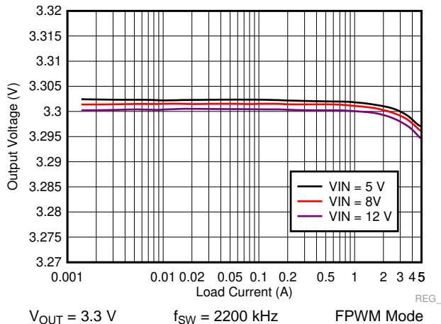
Figure 46. LM73605 Load and Line Regulation
