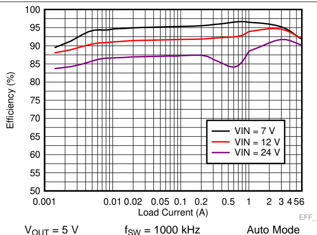
Figure 35. LM73606 Efficiency
