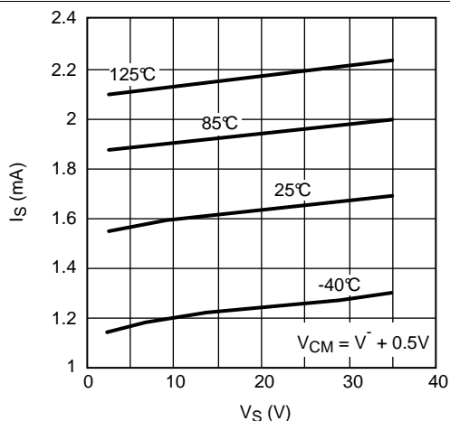
Figure 17. I_S vs Supply Voltage
